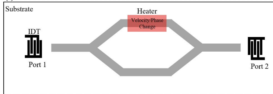
Schematic of all acoustic (a) waveguide (b) 50:50 splitter, (c) phase shifter
