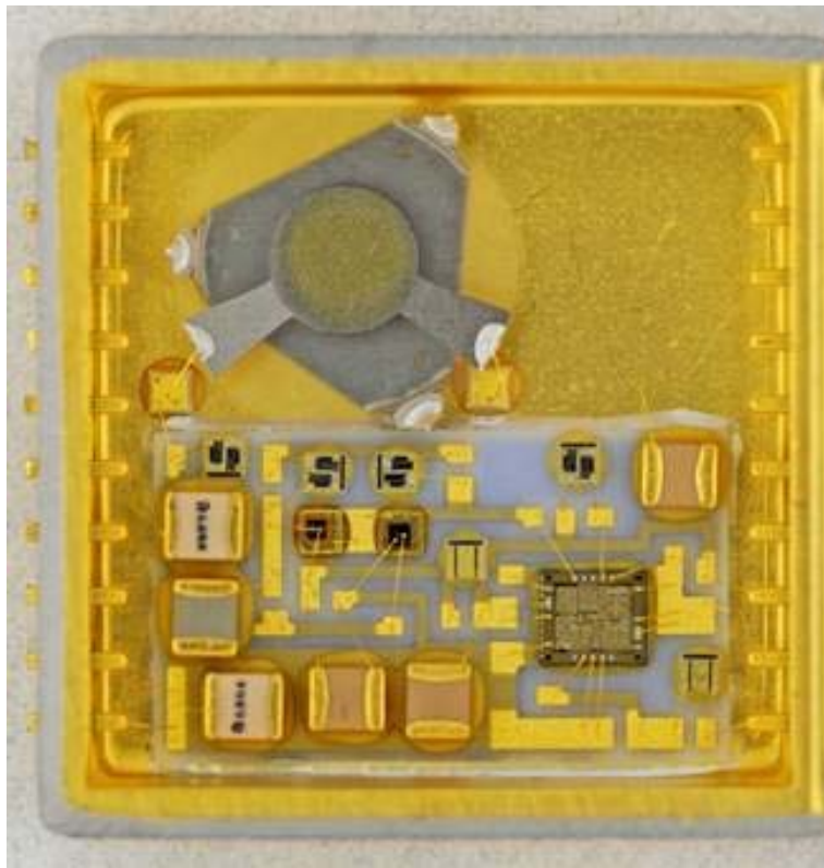
Figure 1. Photo of a typical crystal oscillator, containing an exposed crystal element (upper left) along with the discrete passive components, discrete active components, and an integrated circuit chip (lower right) characteristic of a hybrid microcircuit. (Image from JPL Destructive Physical Analysis report 11036 (internal report).)
