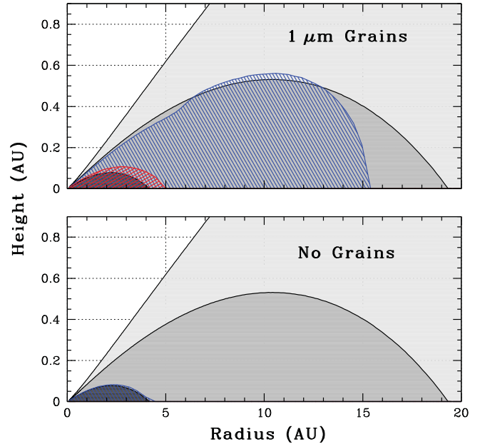
FIG. 1.—Location of the dead zone (red) and undead zone (blue) in a cross-section view of the minimum-mass protosolar disk. The dead zone gas is decoupled from the magnetic fields, while the undead zone is sufficiently ionized for the generation of toroidal fields by shear. The remainder of the disk body is well coupled to the fields and is turbulent through magnetorotational instability. The star lies at the origin, the disk midplane falls along the horizontal axis, and solid black contours show vertical mass columns of 1, 10, and 100 \text{g cm}^{-2} . The pressure in the vertical component of the magnetic field is set to 0.1% of the midplane gas pressure. The ionization is due to stellar X-rays and the decay of radioactive ^{26}\text{Al} . Recombination on grain surfaces is included in the calculation shown at top, where the dead zone extends to 5 AU in the midplane. The grains are 1 \mu\text{m} in radius and well mixed in the gas at a 1% mass fraction. With the grains removed, there is no dead zone (bottom panel).
