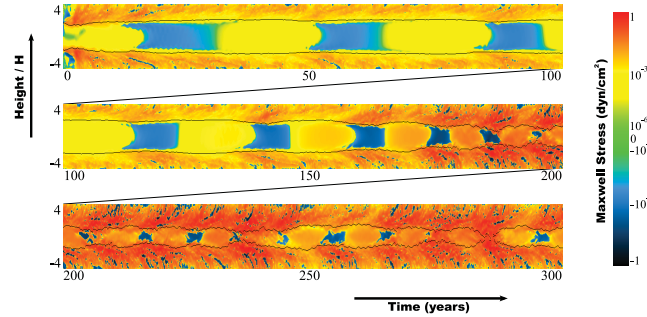
FIG. 3.—Magnetic accretion stress vs. height and time in a resistive MHD calculation of a patch of the protosolar disk at 1 AU. The stress is proportional to the radial and toroidal components of the magnetic field. It is horizontally averaged across the patch and is plotted using a double-logarithmic color scale, with outward angular momentum transport in red and yellow, and inward transport in black and blue. The calculation lasts 300 yr and each panel shows a 100 yr interval. Black curves mark the edges of the undead zone where the resistivity suppresses magnetorotational turbulence. Magnetic activity in the undead zone is driven by the diffusion of magnetic fields from the turbulent surface layers. After 150 yr, the activity grows stronger due to an increase in magnetic coupling as ionized gas is mixed from the surface layers toward the midplane.
