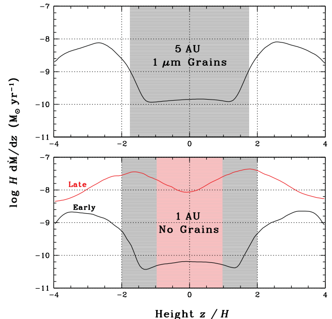
FIG. 4.—Accretion rate corresponding to the total stress in the two MHD calculations located at 5 AU (top) and 1 AU (bottom). The accretion rate per density scale height H is plotted against the distance z from the midplane. The results are averaged from 20 to 120 orbits (solid black curves at top and bottom) and after mixing reduces the size of the undead zone, from 200 to 300 orbits (red curve in bottom panel). The vertically integrated accretion rates are 2.2 \times 10^{-8} , 6.4 \times 10^{-9} , and 1.5 \times 10^{-7} M_{\odot} \text{ yr}^{-1} , respectively. Shading of the same colors marks the undead zone.
