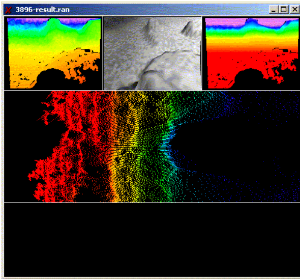
Fig 12. Output of JPL Stereo operating on ROAMS imagery. The top corners show range data coloured by distance and by elevation. Dense, undistorted range output suggests that the imagery is geometrically consistent with the camera model used to generate the stereo.
