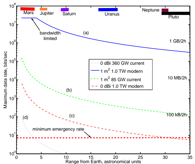
Fig. 1: Present and future transmission performance at 7.2 GHz. (a,b): Routine transmission with space antenna effective area 1.0 m 2 . (c,d): Emergency transmission with omnidirectional space antenna. (a,c): Modern spacecraft electronics and 1.0 TW earth station; error correction code for routine case only. (b,d): Existing spacecraft electronics, 85 GW routine, 360 GW emergency, no coding.
