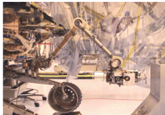
Figure 4. Robotic arm (Instrument Deployment Device)
