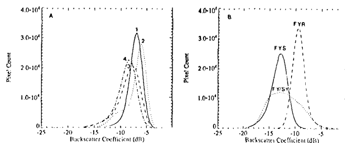
Figure 4. Calibrated ERS-1 SAR image histograms for (a) summer second-year ice around ISW-1 under varying wind and temperature conditions; and (b) winter first-year smooth (FYS), first-year rough (FYR) and mixed first- and second-year ice (FY/SY).
