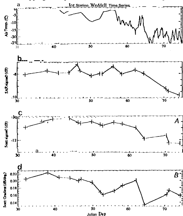
Figure 6. Comparison of ISW-1 temperature record with C-band SAR ( 20-27^\circ ) and Scatterometer backscatter time-series ( 40^\circ ) data.
