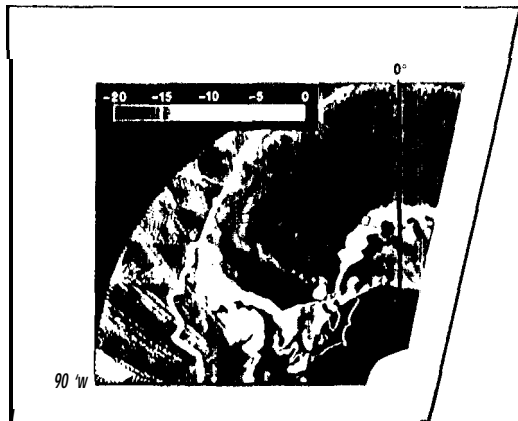
Figure 3. Enhanced resolution ERS-1 Scatterometer image of the Weddell Sea sector of the Southern Ocean during winter. Locations of SAR image data arc shown by open boxes.
