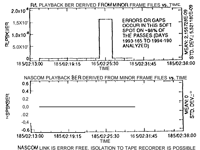
Figure 4.4. Tape Recorder C BER Signature
