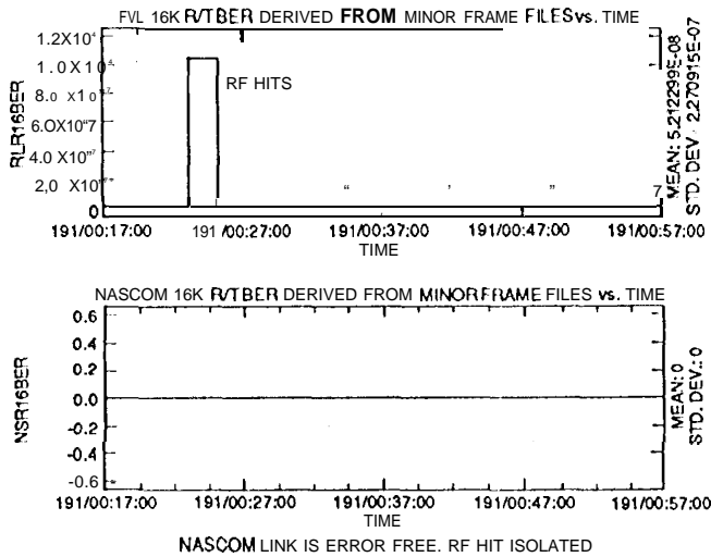
Figure 4.2. MONITOR_MA Pass (1993-191) Showing RF Bit Errors
