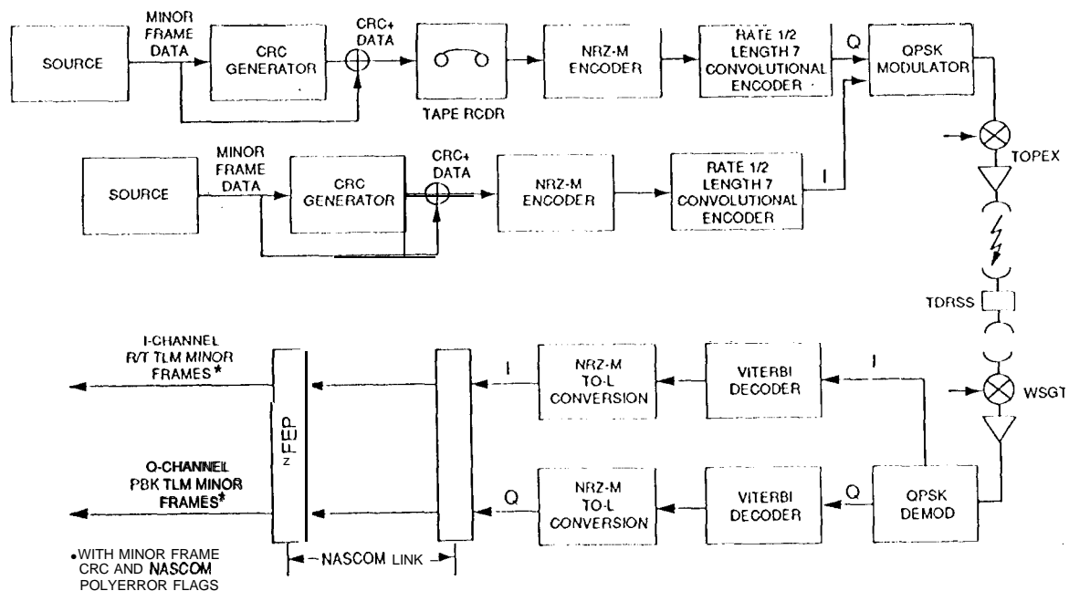
Figure 2.2. TOPEX Data Transmission/Recovery Scheme 1
