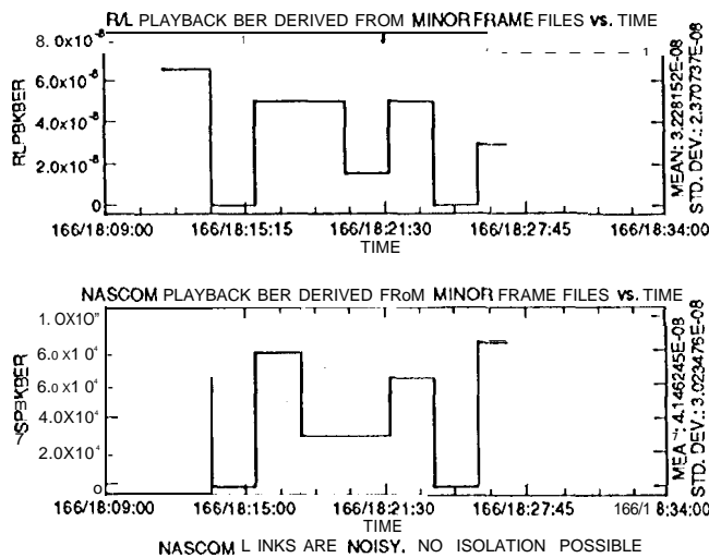
Figure 4.3. NASCOM Link Errors Coupling Onto the Received Playback Minor Frames (Tape Recorder B Playback)
