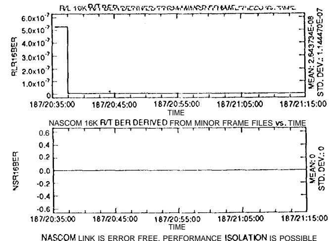
Figure 4.1. Typical LOAD_MRO_SA Performance (Day 1994-187)
