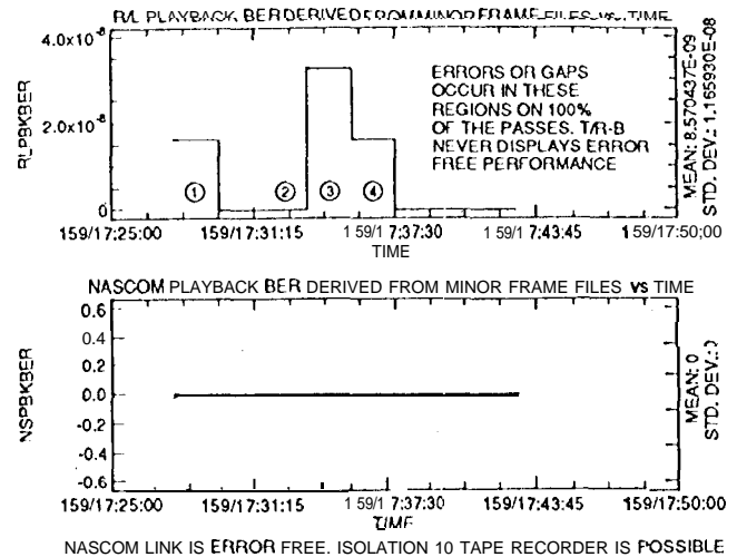
Figure 4.6. One of Many Tape Recorder B Signatures (All Soft Spots Are Shown)
