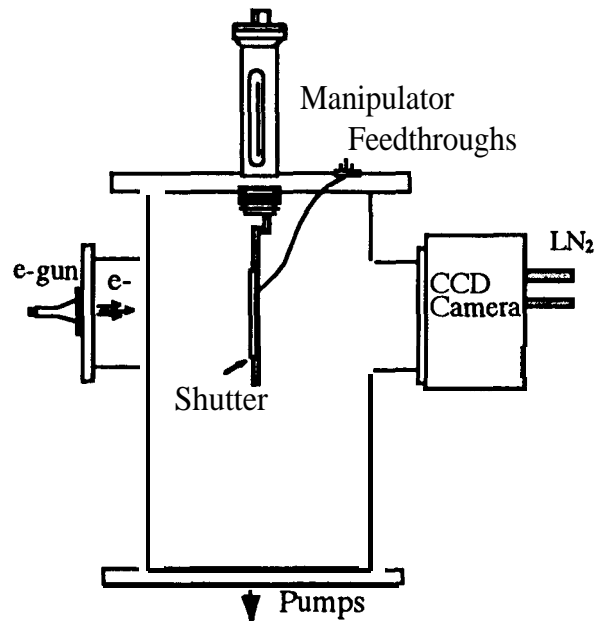
Figure 4b. UHV chamber used in the imaging mode.
