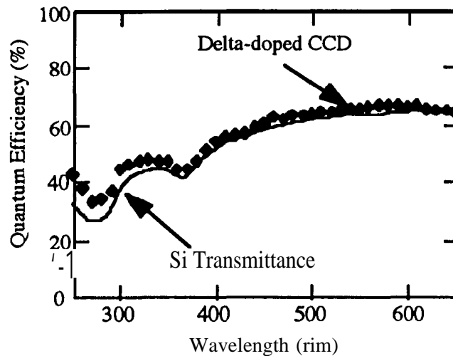
Figure 3 Typical quantum efficiency of delta-doped CCDs. Comparison with the reflection-limited quantum efficiency (transmittance of silicon) shows that the delta-doped CCDs exhibit nearly 100% internal quantum efficiency.
