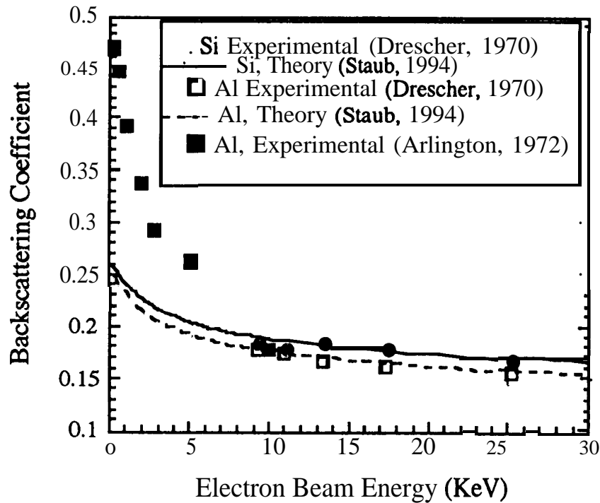
Figure 6. Experimental and theoretical backscattering results with extrapolation down to 200 eV.
