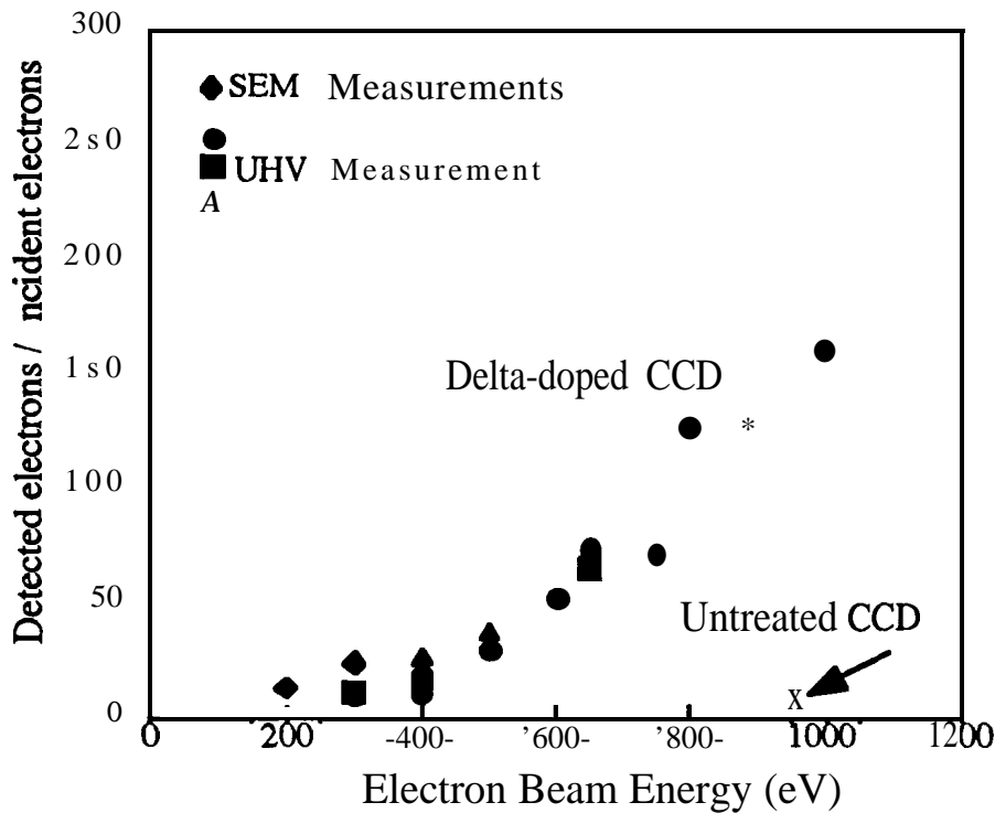
Figure 5. Quantum efficiency of delta-doped CCD with low-energy electrons using SEM and a indirectly-heated cathode gun. The increase in the QE with energy is the result of multiple electron-hole pair generation. The response of the untreated CCD has been plotted for comparison.
