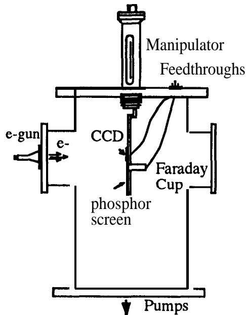
Figure 4a. UHV chamber used in the photodiode mode.
