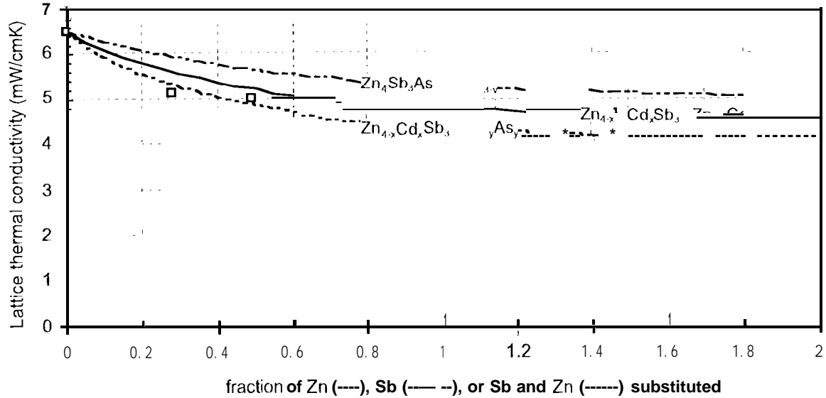
FIG. 2. Effect of alloy scattering on the room temperature lattice thermal conductivity of \beta - \text{Zn}_4\text{Sb}_3 . The values were calculated as a function of the fraction x for \text{Zn}_{4-x}\text{Cd}_x\text{Sb}_3 alloys ( x_{\text{max}} = 2 ) and y in \text{Zn}_4\text{Sb}_{3-y}\text{As}_y alloys ( y_{\text{max}} = 1.5 ). For \text{Zn}_{4-x}\text{Cd}_x\text{Sb}_{3-y}\text{As}_y alloys, the calculated values reflect a scaling of y_{\text{max}} to a value of 2. The symbol \square denotes experimental data for \text{Zn}_{4-x}\text{Cd}_x\text{Sb}_3 alloys.
