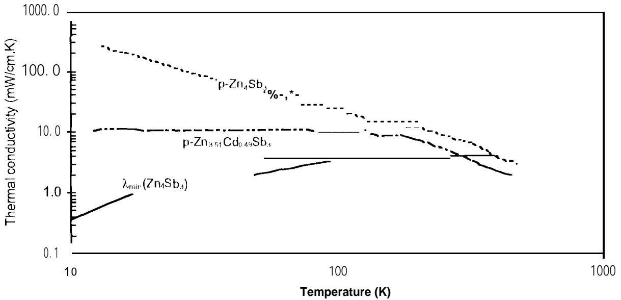
FIG.3. Lattice thermal conductivity vs. temperature for p-type \beta - Zn_4Sb_3 and p-type Zn_{3.51}Cd_{0.49}Sb_3 alloy. The solid line is the calculated lattice thermal conductivity for \beta - Zn_4Sb_3 using equation (1),
