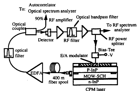
Fig. 4 The cross-section illustration of a colliding pulse mode-locked laser and a COEO constructed with the laser.
