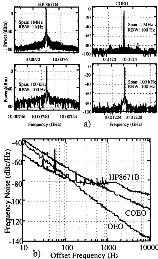
Fig. 3 a) Measured RF spectra of the COEO output at different spectrum analyzer settings and the comparison with a signal from a HP8671B synthesizer. b) Single sideband phase noise comparison of the COEO, a OEO and a HP 8671B synthesizer at 10 GHz.
