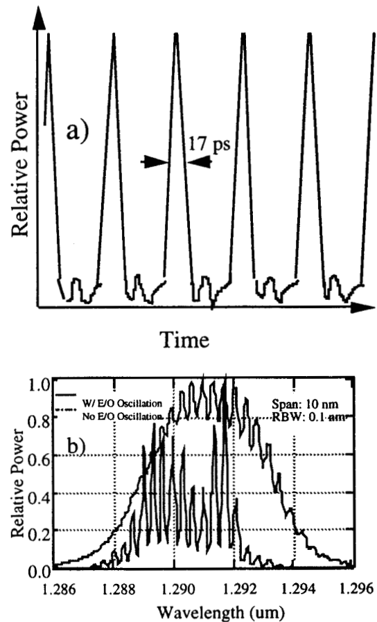
Fig. 2 a) Time domain measurement of the optical pulses. b) Optical spectrum of the ring laser with (upper curve) and without opto-electronic oscillation.
