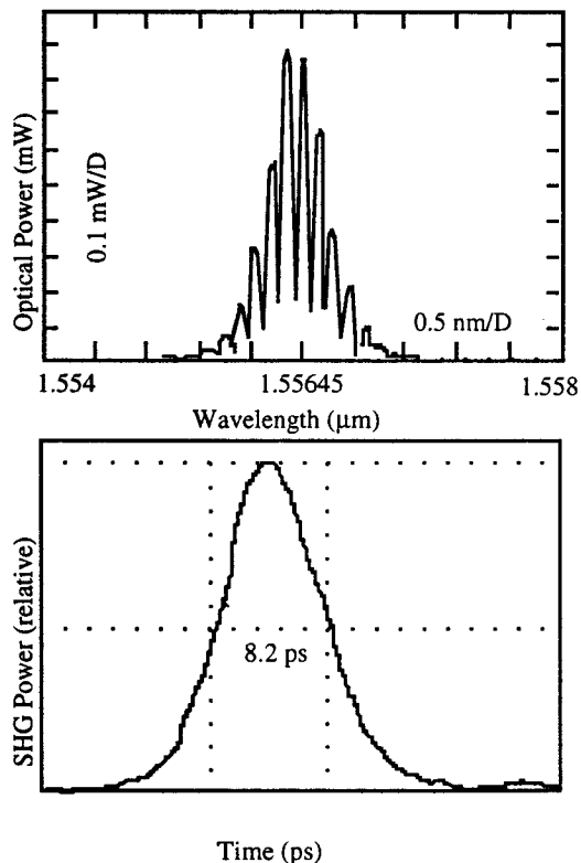
Fig. 5 a) The optical spectrum of a pulse train from a CPM laser based COEO. b) the auto-correlation measurement of the pulse train.
