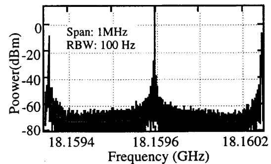
Fig. 6. RF spectrum measurements of a COEO constructed with a CPM laser.
