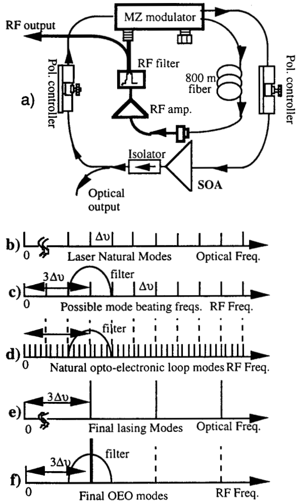
Fig. 1 a) Illustration of a COEO constructed with a SOA and a Mach-Zehnder modulator. b) All possible laser modes with a mode spacing of \Delta\nu . They have random phases in the absence of the electro-optic feedback. c) All possible mode beat frequencies of the laser modes in the photodetector. The lowest frequency ( \Delta\nu ) corresponds to the sum of the beats between adjacent modes, the second lowest frequency ( 2\Delta\nu ) corresponds to the sum of the beats between every other modes, and so on. Due to the random phases of the laser modes, these beat signals are weak and noisy. d) All possible oscillating modes defined by the opto-electronic loop. Only those modes aligned with a mode beat frequency can get gain (or energy) from the laser. An electrical filter
