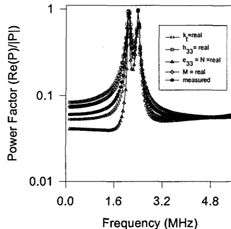
Figure 4. Electrical power factor for the measured resonator and assuming lossless material constants
