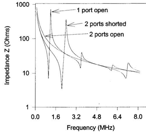
Figure 2. A comparison of the analytical solution, Mason's and the KLM model under various acoustic boundary conditions. All models were found to overlap.
