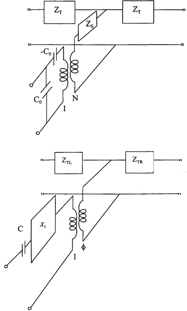
Figure 1. KLM and Mason's equivalent circuits. Quantities in figure are defined in Table 1.
