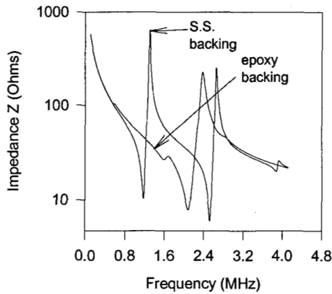
Figure 3. A comparison of the analytical solution, Mason's and the KLM model with stainless steel and epoxy backing layers. All models were found to overlap.
