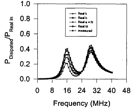
Figure 5. The electrical power dissipated in the piezoelectric element of the transducer described in text for k_t measured, k_t real, e_{33} \propto N real, h_{33} real., and M real.
