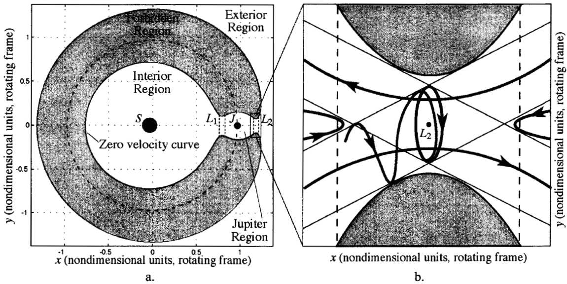
Figure 2a. The Hill's Region Connecting the Interior (S), the Planet (J), and the Exterior (X) Regions. 2b. Expanded view of the L2 Region with 4 Major Classes of Orbits: Black – Lyapunov Orbit (Unique for Each Energy Level) Red – Transit Orbits (Must Pass Thru Lyapunov Orbit) Green – Spiral Orbits (The Manifolds, Form Tubes), Blue – Non-Transit Orbits.
