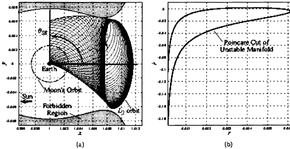
Figure 4. The Sun-Earth Unstable Manifold (Red) (a) and Its Poincaré Section (b).
