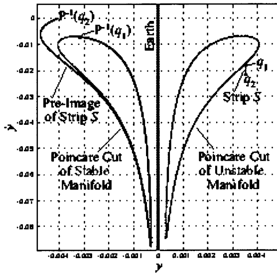
Figure 5. Using the Poincaré Section to Find the Transfer Trajectory.
