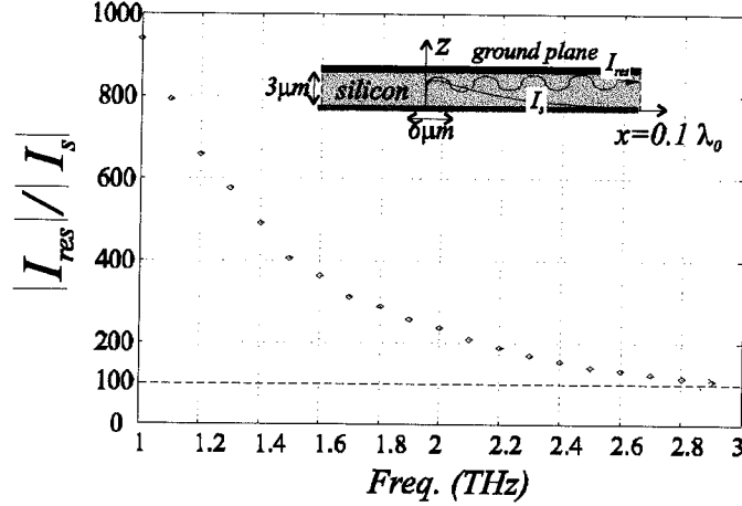
Fig. 9 Ratio between the amplitudes of the residue contribution to the currents and the source attached currents. The graph can be read as 1/(A(l=0.1\lambda_0)) . The microstrip impedance is nominally 50 ohm. The width of the microstrip and the thickness of the dielectric are 2.5 \mu\text{m} and 3 \mu\text{m} respectively. The grounded dielectric is made of silicon ( \epsilon_{r1}=11.7 ). The width of the gap is \lambda_0/40 .
