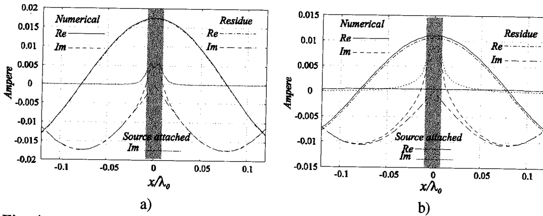
Fig. 4 Comparison between asymptotic evaluation (residue only) and direct numerical integration of the current for a sample microstrip structure at submillimeter wave frequencies (2.5 THz). Also plotted is the source attached field (real and imaginary parts in 4.b and only the imaginary part in 4.a since the real part is almost zero and cannot be distinguished in the drawing scale). The width of the microstrip and the dimensions of the excitation gap ( \delta ) are \lambda_0/20 ( 6\mu\text{m} ), \lambda_0/60 ( 2\mu\text{m} ) respectively. The height of the slab is \lambda_0/40 ( 3\mu\text{m} ) in Fig. 4a and \lambda_0/20 ( 6\mu\text{m} ) in Fig. 4b. The relative dielectric constant considered is ( \epsilon_{r1} = 12.85 ).
