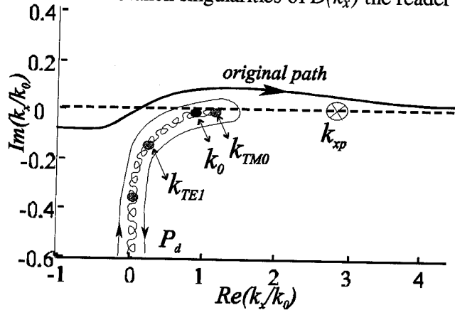
Fig. 2 Complex k_x plane topology for thin dielectric substrates. Only the TMO pole of the grounded slab is assumed to be above cut off.
