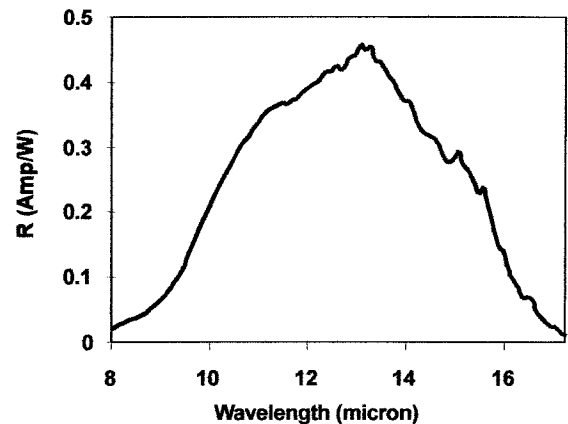
Fig. 1. Responsivity spectrum of a broadband QWIP test structure at temperature T = 55 \text{ K} . The spectral response peak is at 13.5 \mu\text{m} and the long wavelength cutoff is at 15.4 \mu\text{m}
