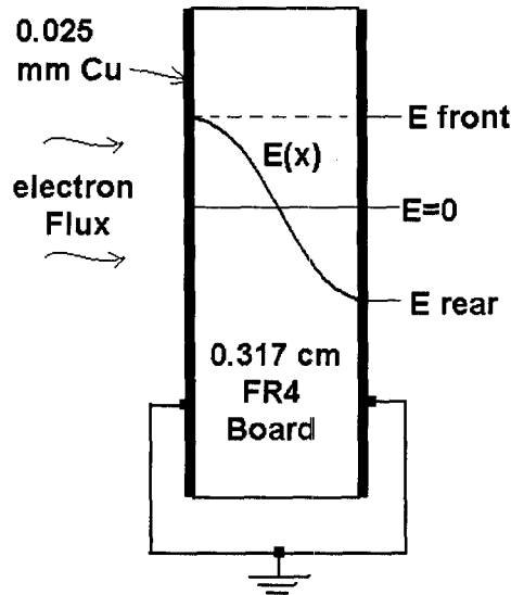
Figure 2. Description of Electric Field Profile in Geometry #4 on CRRES/IDM.
