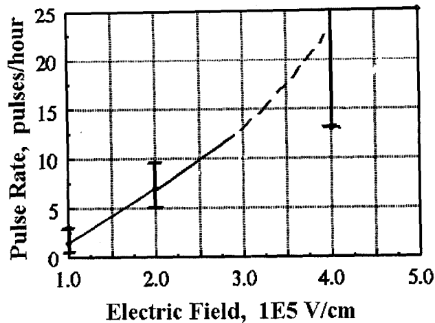
Figure 9. Pulse Rate on FR4 Board in 30 keV Ground Tests.
