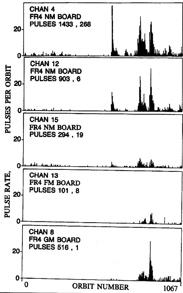
Figure 7. Pulse Rates for the FR4 Circuit Board Samples on CRRES/IDM.
