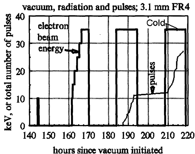
Figure 6. Vacuum and keV Electron Exposure History of the FR4 Sample. When the beam was on, the flux was 0.5 \text{ nA/cm}^2 .
