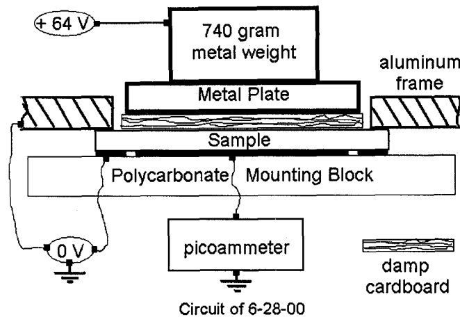
Figure 1. Method for measuring resistivity of the samples. The inner diameter of the guard ring is 4.77 cm. The laminated circular copper electrode at the bottom of the sample has area of 16.6 cm 2 . The sample thickness is 0.0051 cm. The test was performed in room air. Voltage was varied from +64V to -64V.
