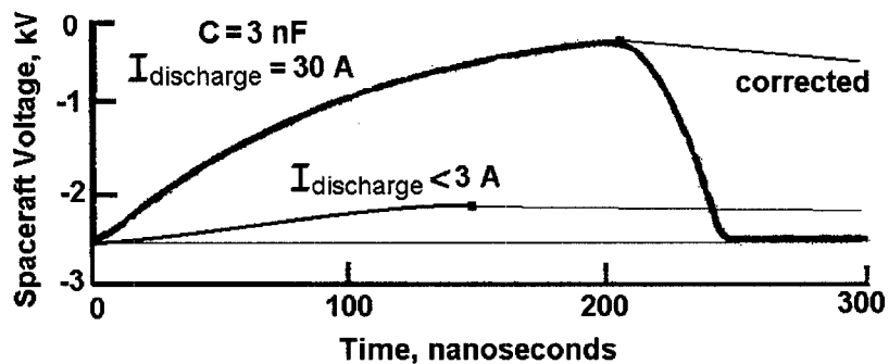
Figure 13. Predicted Discharge Current from NASA TP-2361. A large spacecraft would require a 3 nF capacitance to space plasma ground to produce the 30-A discharge in Fig. 8 of NASA TP-2361. Assuming this to be possible, lab tests of MLI and OSR have measured discharge currents of 30 A provided that the electric field in the MLI is very high. However, in what are now believed to be more representative spacecraft arcing configurations, recent lab tests imply that the pulses will be like the lower curve in the figure--e.g., smaller than 3 A. Realistic internal fields produce the smaller pulses. Furthermore, when spacecraft are at high charging voltage they are often at low capacitance to plasma, thus reducing the discharge to space even more severely.
