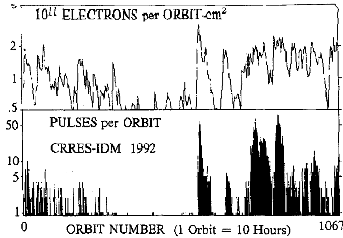
Figure 3. High-energy Electron Flux incident on the Samples over the Life of CRRES, 1067 Orbits, and Pulse History Summed Over All CRRES/IDM Samples. [4]
