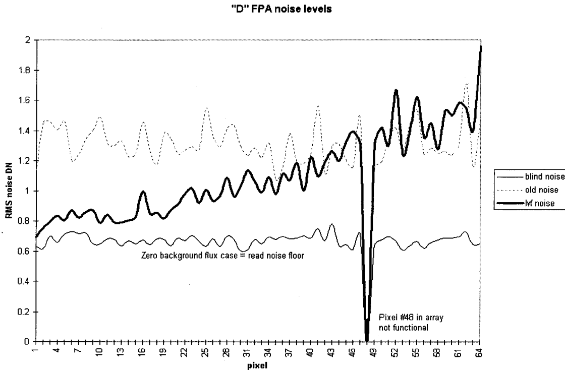
Figure 2. "D" FPA noise levels for cold-blind case, 1997 passband blocking filter lab bench case (on-AVIRIS noise level 30% higher), and Linear Variable Blocking Filter background-reduced case.
