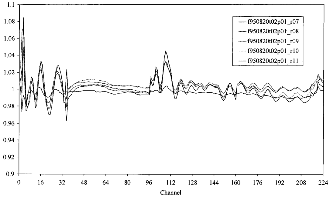
Figure 5. Ratio of consecutive measurement from a stable source to the first measurement for a series of AVIRIS data sets in 1995.
