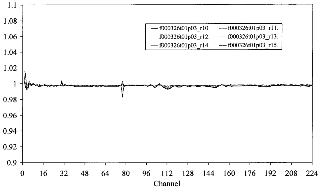
Figure 7. Ratio of consecutive measurement from a stable source to the first measurement for a series of AVIRIS data sets in 2000.
