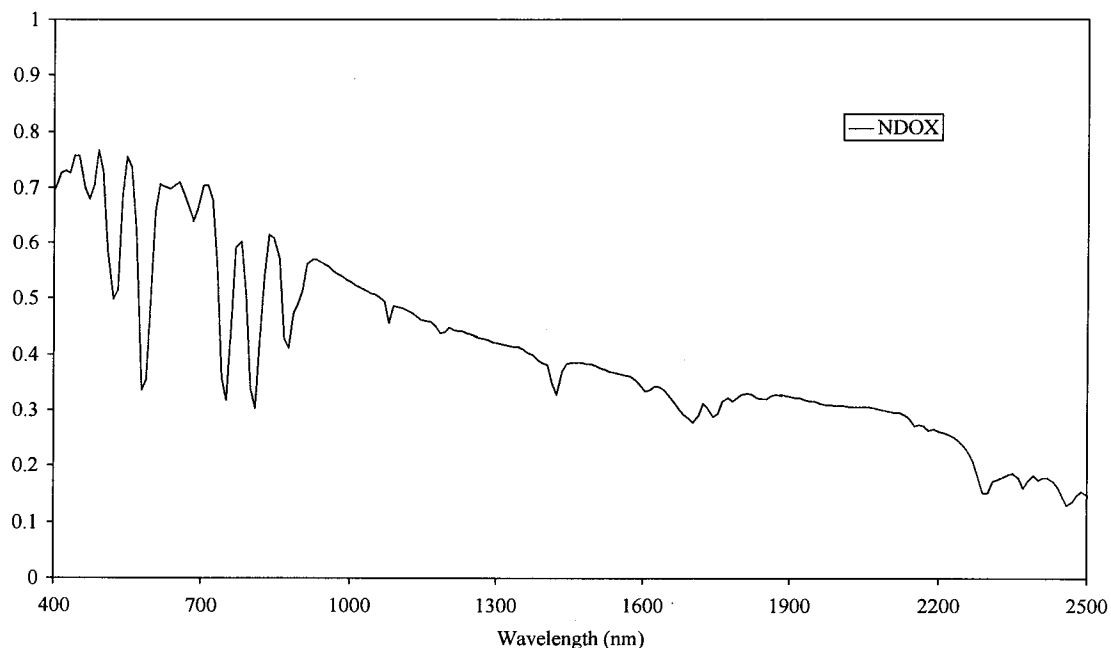
Figure 8. Ratio of the NdOx coated side of the AVIRIS foreoptics shutter to the uncoated side. This is the spectral calibration signal of the AVIRIS onboard calibrator.
