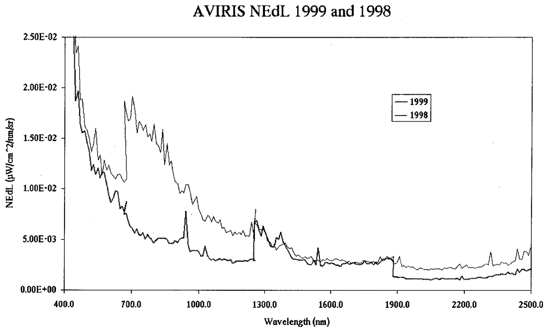
Figure 4. AVIRIS NEdL improved dramatically in the B range due to the combination of an optimized hybrid silicon + InGaAs photodetector array and the improved multiplexer performance. C did not improve due to the inclusion of non-QE-optimized InSb in the reworked C FPA.
