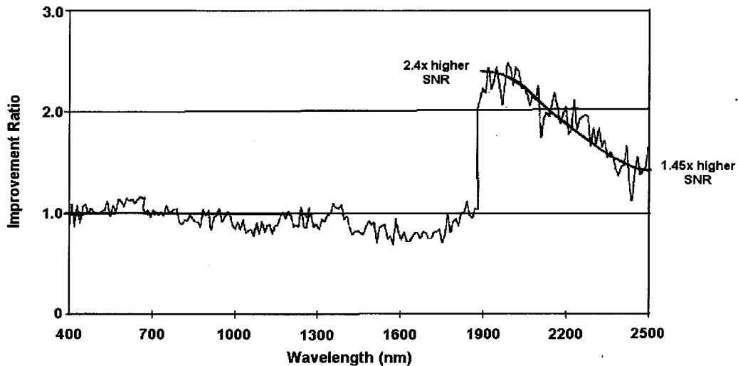
Figure 3. Ratio of 1998 to 1997 AVIRIS pre-season laboratory signal-to-noise performance showing combined effect of new linear variable blocking filter, plus system grounding noise reduction.
