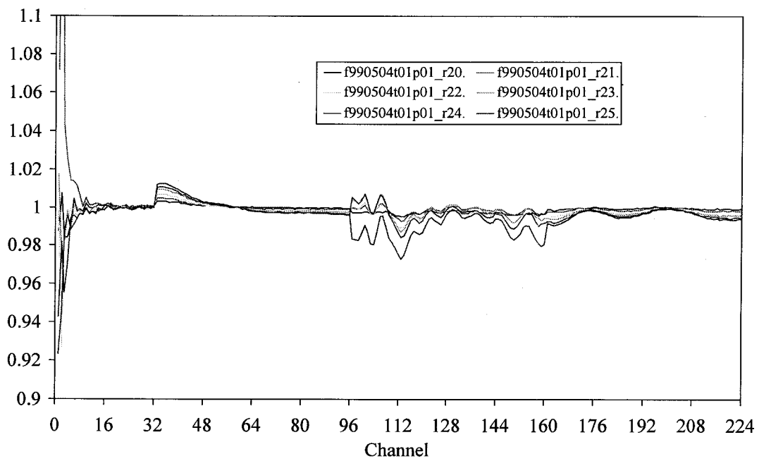
Figure 6. Ratio of consecutive measurement from a stable source to the first measurement for a series of AVIRIS data sets in 1999.
