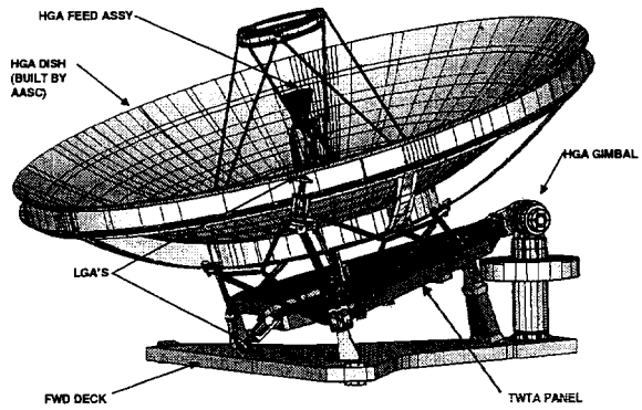
SLJ Radome, MLI Dish Blanket, and TWTA Assy. Blanket not shown
