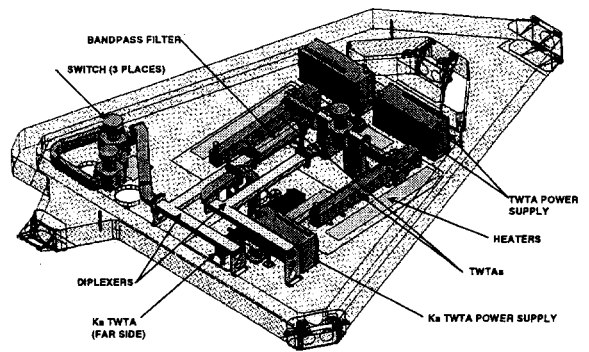
FIGURE 5. TWTA ASSEMBLY
