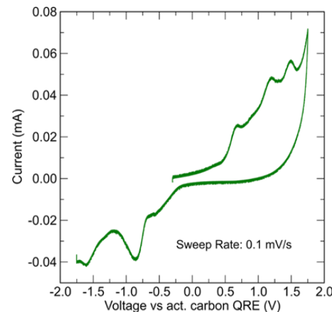
Cyclic voltammogram of \text{Sr}_2\text{FeO}_3\text{F}
