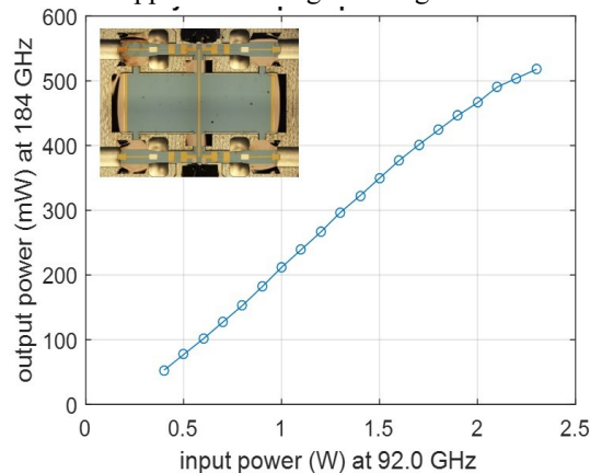
Figure 1: Novel chip topologies have now enabled relatively high power sources in THz range. This particular chip provides over 500 mW at 184 GHz.
