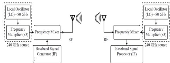
Figure 3: Advanced THz components are utilized for a broadband communication link at 240 GHz.
