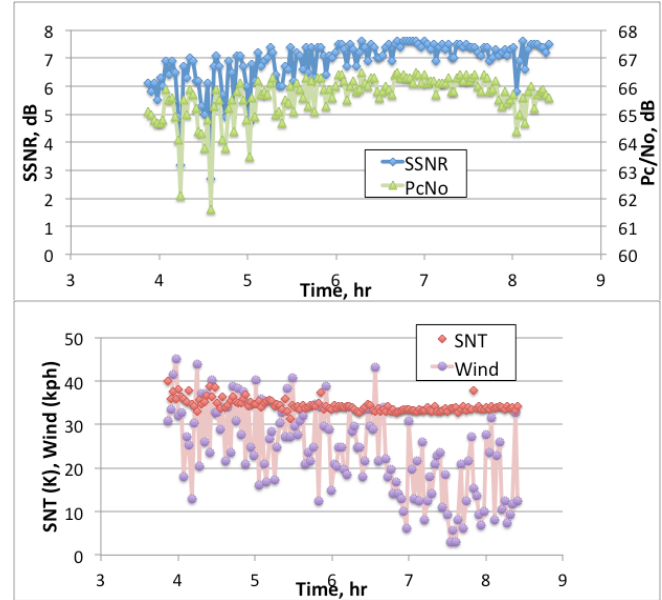
Figure 5. Variation of SNR, system noise temperature and wind speed on DOY243/DSS-34
