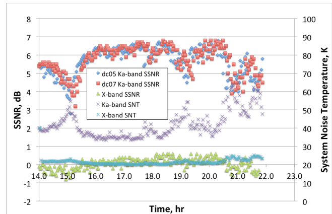
Figure 3. Variation of symbol SNR and system noise temperature at Ka- and X-band on DOY32/DSS-55
