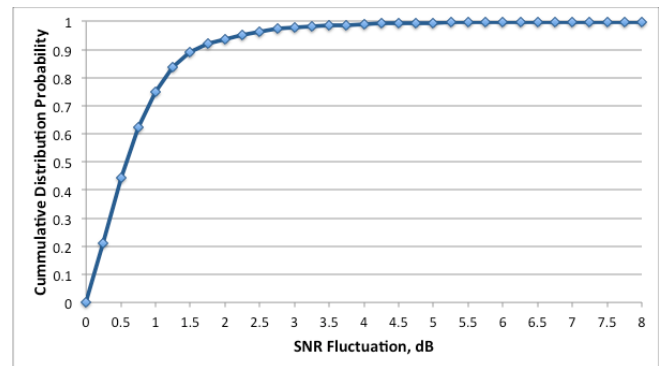
Figure 9. Cumulative distribution of SNR fluctuation
