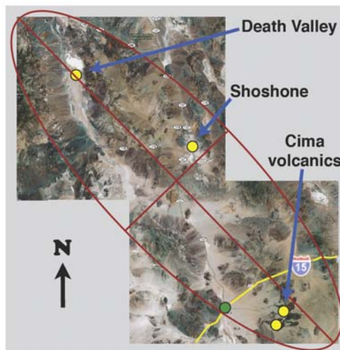
Figure 2. Sites within the Mojave Desert National Preserve & Death Valley National Park. Pale gold dots are proposed drill sites (northern site is DV; southern sites are Cima volcanics; middle site is near Shoshone, CA). Green dot is Baker, CA. Major axis of hypothetical landing ellipse is 100 km.
