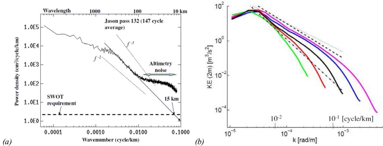
Figure 1. (a) Spectrum of sea surface height anomaly from Jason altimeter data (solid line). The two slanted dashed lines represent two spectral power laws with k as wavenumber. The horizontal dashed line represents the proposed SWOT requirement of measurement noise at 1/km sampling rate. The slanting solid straight line represents a linear fit of the spectrum between 0.002 and 0.01 cycles/km. It intersects with the threshold noise level at 15 km wavelength [4]. (b) Wavenumber spectra for simulated kinetic energy at 10- m depth. Straight lines indicate -5/3 (dotted), -2 (dashed), and -3 (dot-dash) spectrum slopes. The five other lines correspond to different simulations whose resolutions increase from 12 (green), 6 (red), 3 (black), 1.5 (blue) to 0.75 km (purple) [5].
