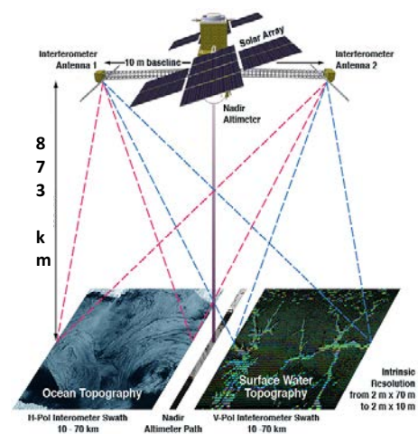
Figure 5. A schematic illustration of the measurement configuration of the proposed SWOT Mission
