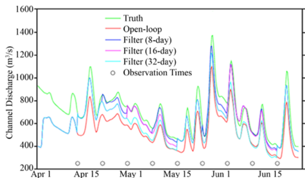
Figure 4. Discharge estimates from assimilating synthetic SWOT observations into a hydrodynamic model of the Ohio River for different repeat times (top; [11]).
