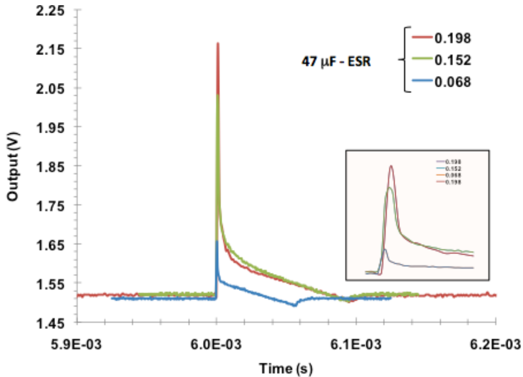
Figure 3.2-1. Impact of ESR on the regulator SET response for a fixed output capacitor and load current. The MSK5920RH was tested for SET with a V_{in} of 5 V, V_{out} of 1.5 V, a load of 50 mA, and a capacitive value of 47 \mu\text{F} . The capacitive load ESR was varied: 68, 152, and 198 m \Omega . SET magnitude and duration were observed to increase with increasing ESR.
