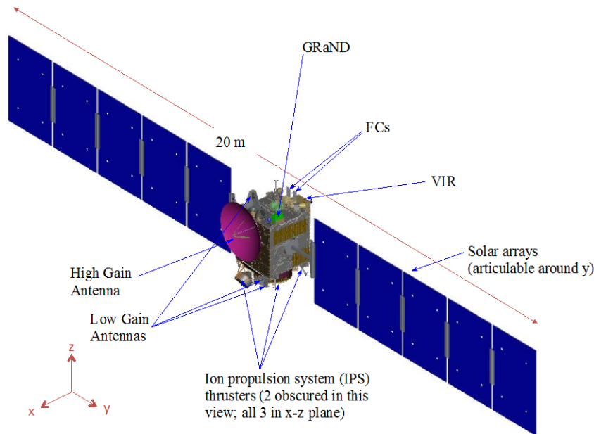
Figure 2. Dawn Spacecraft
