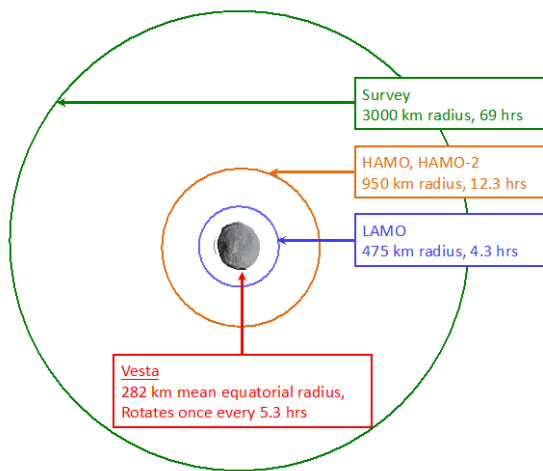
Figure 3. Vesta Orbits
