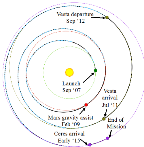
Figure 1. Dawn's interplanetary trajectory
