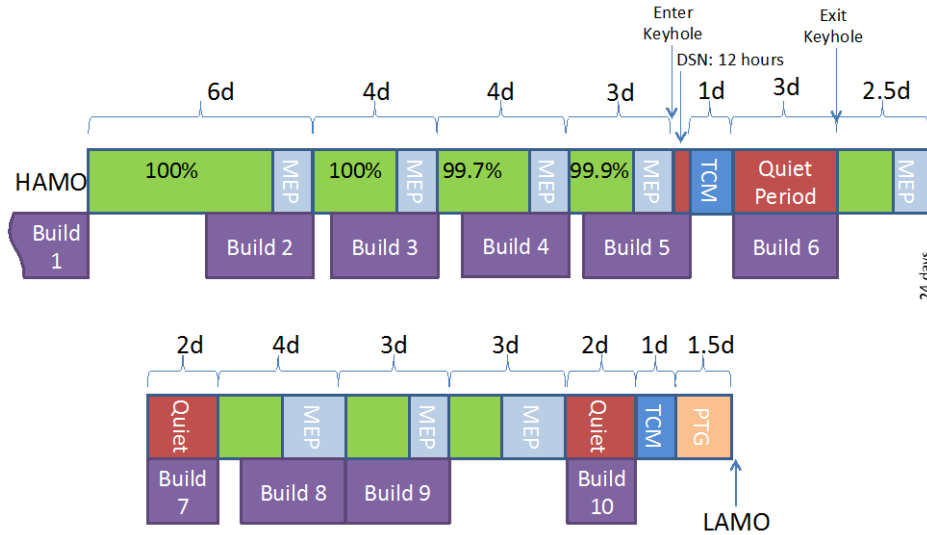
Figure 6. HAMO to LAMO transfer architecture
