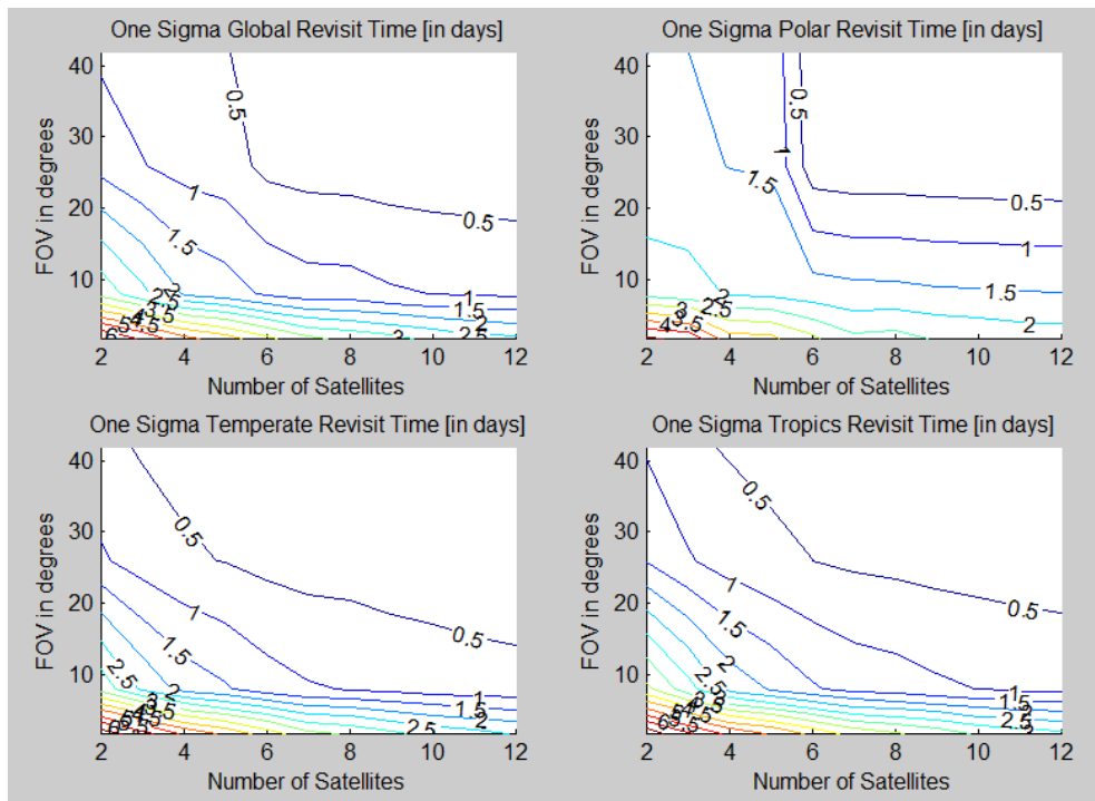
Figure 6: 1 sigma time between ground revisit in number of days as a function of instrument FOV and number of satellites in a randomly selected ad-hoc constellation. The 1 sigma value is chosen from the results obtained over 50 Monte Carlo runs performed using the parameters in Table 2. The results are divided in to 4 geographic regions: Global, Polar, Temperate, and Tropics. Definitions for these regions can be found in Table 1.
