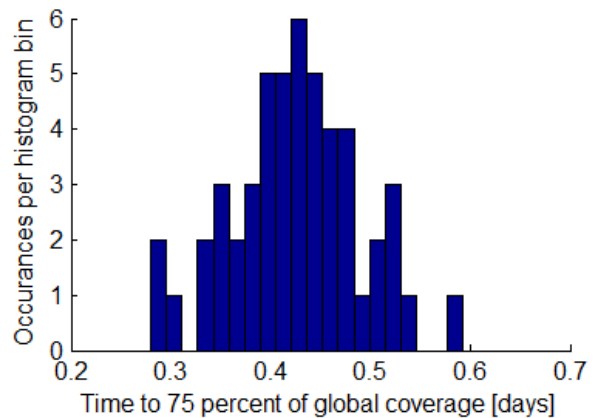
Figure 4: For FOV 25.9° and 8 satellite constellation. This histogram shows the distribution of coverage FOM for all 50 Monte Carlo runs. Note that the 68 th percentile value is at 0.5 day revisit, consistent with the value in Figure 5
