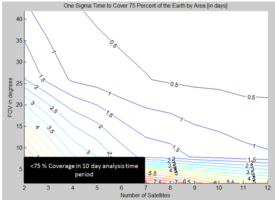
Figure 5: 1 sigma time of ground coverage for 75% of the Earth’s surface as a function of instrument FOV and number of satellites in a randomly selected ad-hoc constellation. The 1 sigma value is chosen from the results obtained over 50 Monte Carlo runs performed using the parameters in Table 2
