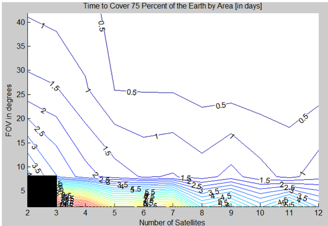
Figure 7: Time of ground coverage for 75% of the Earth’s surface as a function of instrument FOV and number of satellites in a Walker constellation. The parameters of the Walker constellation are shown in Table 3. The black region did not achieve 75% coverage within the 10 day analysis period.
