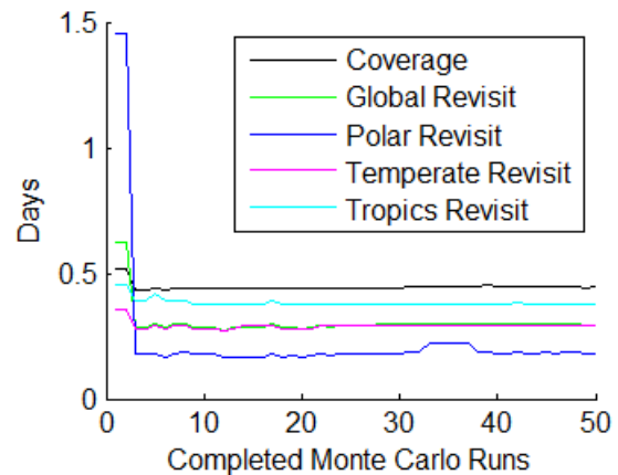
Figure 3: For FOV of 25.9 degrees and an eight-satellite constellation, this plot shows that 50 Monte Carlo runs were sufficient since the analysis has converged to a solution. Similar trends were observed for each of the combinations of FOV and N.
