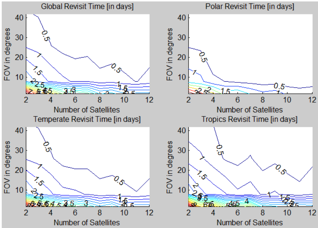
Figure 8: Mean time between ground revisit in number of days as a function of instrument FOV and number of satellites in a Walker constellation. The results are divided in to 4 geographic regions: Global, Polar, Temperate, and Tropics. Definitions for these regions can be found in Table 1. The parameters of the Walker constellation are shown in Table 3.
