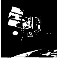
QuikSCAT (1998)
