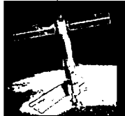
SeaSAT (1978)
