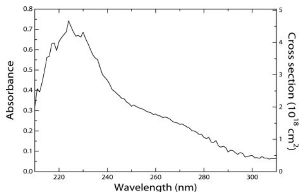
Fig. 2. The UV spectrum of the thermolysis products of CIC(O)OONO 2 at 250°C isolated in a Ne matrix. Computation of a cross section from absorbance is based on an assumption that the yield for FC(O)OO and CIC(O)OO from thermal decomposition of FC(O)OONO 2 and CIC(O)OONO 2 , respectively, is the same under similar experimental circumstances and that the conversion of absorbance to cross section in the FC(O)OO matrix measurements (24) is applicable to the CIC(O)OO matrix measurements.
