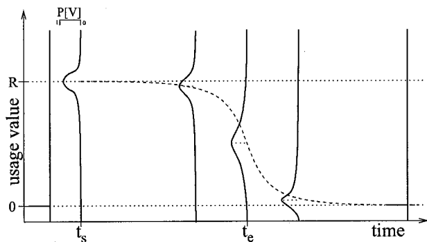
Figure 4: Single peak approximation for resource usage distribution in place of multi-modal distribution (figure 2).
