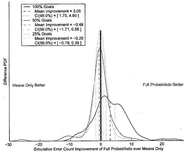
Figure 7: Execution error improvement distribution for problems of different goal densities. (The improvement is measured as the per-problem difference in errors.)
