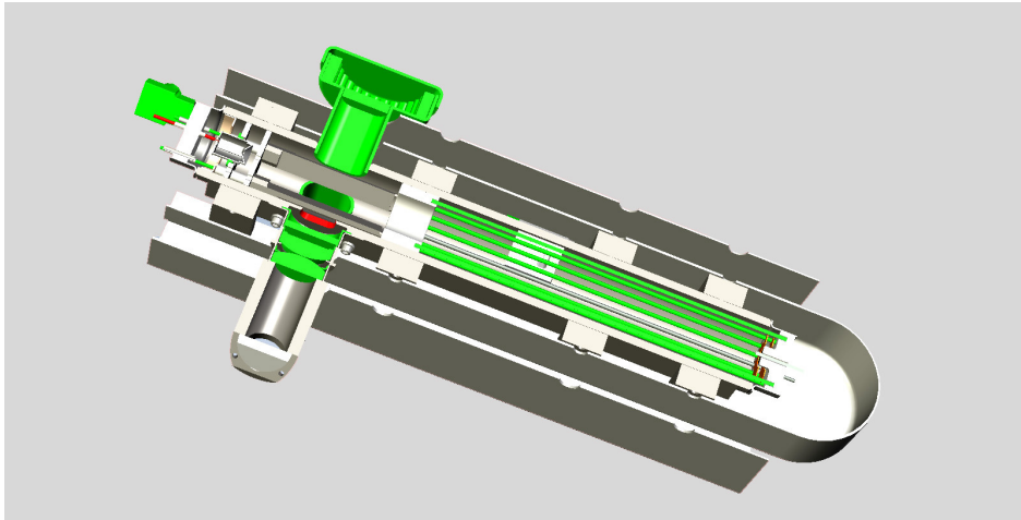
Figure 3. Cutaway design sketch for the 1 liter ion clock physics package layout. The ion tube with 2 layers of magnetic shielding occupies \sim 1/4 of the package volume.
