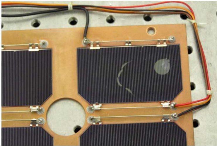
Figure 5. Coverglass "Bubble"
