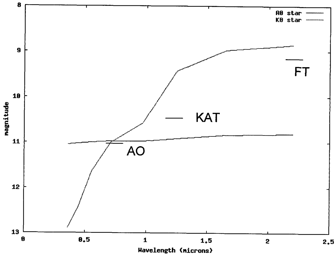
Figure 6. Current limiting magnitudes for the adaptive optics system (AO) at R-band, the angle tracker (KAT) at J-band and the fringe tracker (FT) at K-band. The magnitude versus wavelength for R=11 magnitude A0 and K0 stars is also shown.
