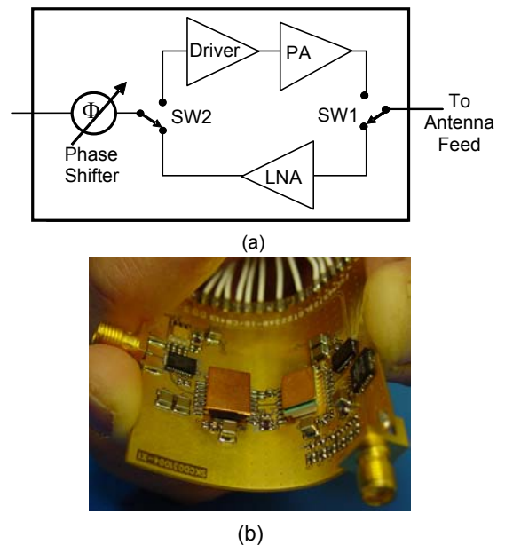
Fig. 3. (a) Block diagram of T/R module. (b) Photograph of the flexible membrane T/R module.
