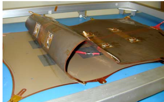
Fig. 6. Antenna in rolled configuration
