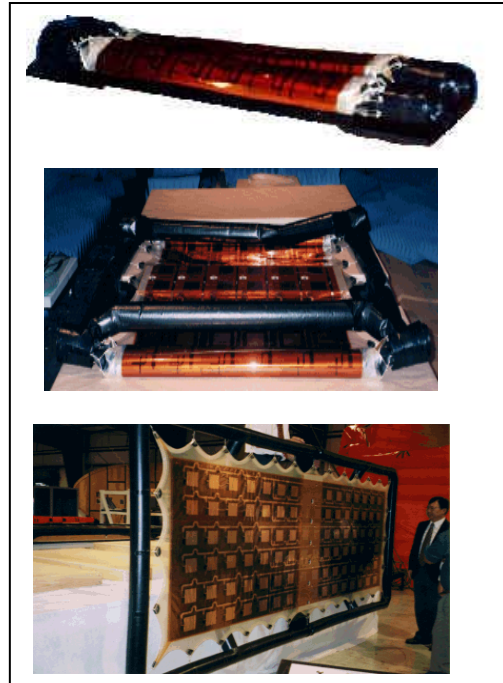
Fig. 1. JPL's 1x3m passive membrane antenna. The top figure shows the antenna in stowed configuration. The antenna is partially deployed in the middle figure. The fully deployed antenna is shown in the bottom.
