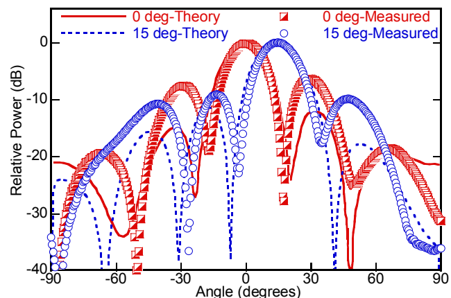
Fig. 9. Transmit antenna patterns for 0^\circ and 15^\circ steering angles.
