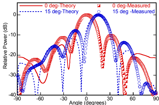
Fig. 8. Receive antenna patterns for 0^\circ and 15^\circ steering angles.
