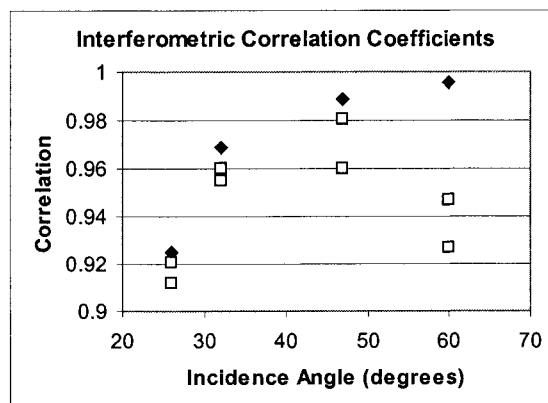
Figure 1. Interferometric correlation coefficients: \gamma_{Scat} (diamond) and \gamma (square).
