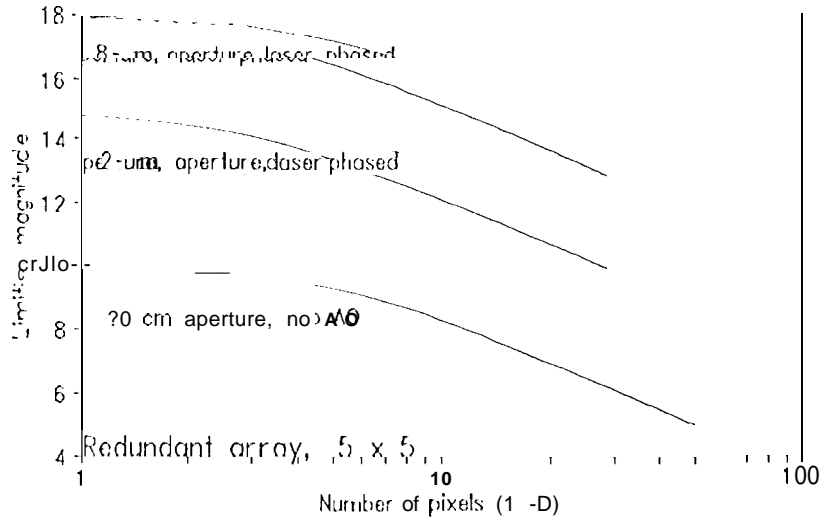
Fig. 1. Approximate sensitivity of a redundant-aperture interferometer ( \sim 5 \times 5 ) for imaging extended objects.
