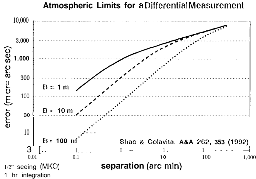
Fig. 2. Error behavior of a differential astrometric measurement as a function of field angle and baseline length.
