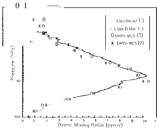
Figure 5, Lidar MLO ozone profile converted to mixing ratio and comparison with two closest UARS overpasses.
