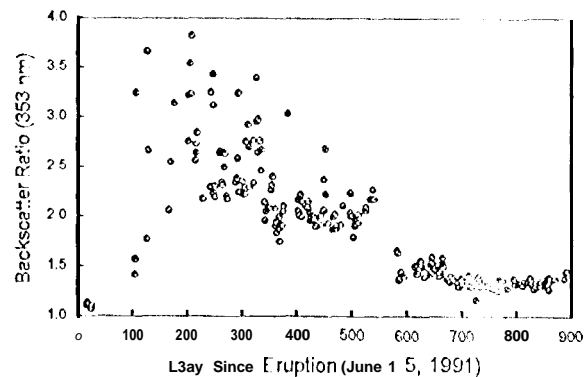
Figure 1. Maximum backscatter ratio at 353 nm as a function of time since the eruption of Mt. Pinatubo.
