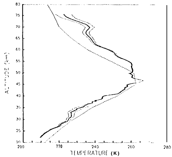
Figure 3. ML0 temperature profile, 1/27/94. Dashed line is CIRA reference atmosphere model.
