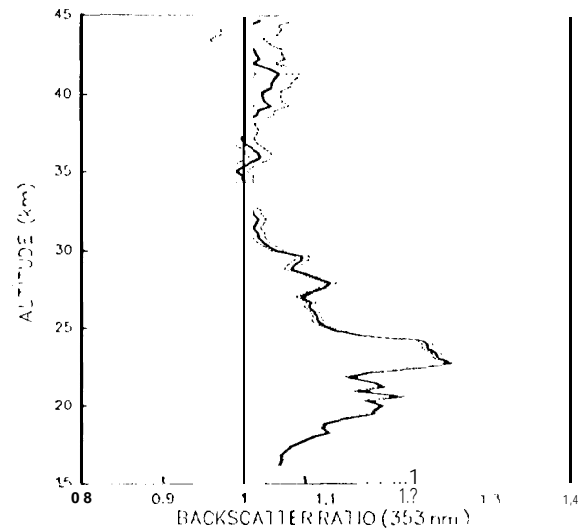
Figure 4. ML0 aerosol profile, 1/27/94
