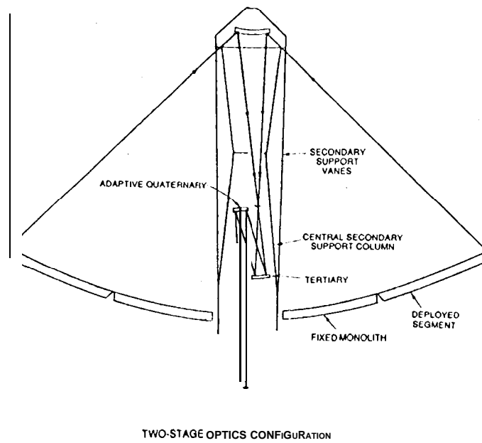
Fig. 4. A possible two-stage optical variant of FAST where wavefront upgrading is done at the small off-axis quaternary mirror.
