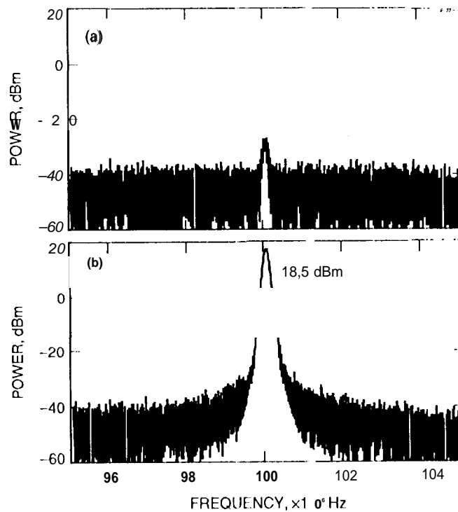
Fig. 10. Carrier recovery measurement in the frequency domain: (a) spoiled carrier and (b) recovered carrier.
