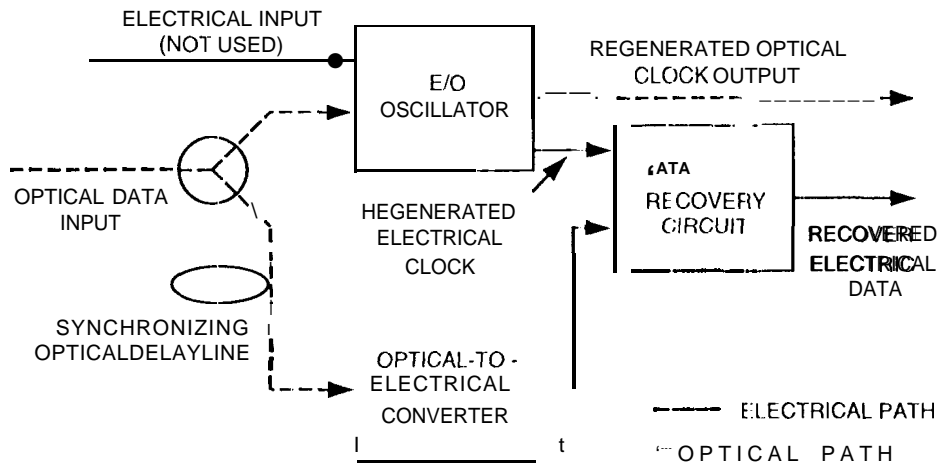
Fig. 12. Clock regenerator and data recovery system.
