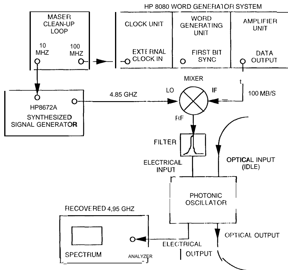
Fig. 7. Experiment setup for clock recovery at 4.95 GHz.
