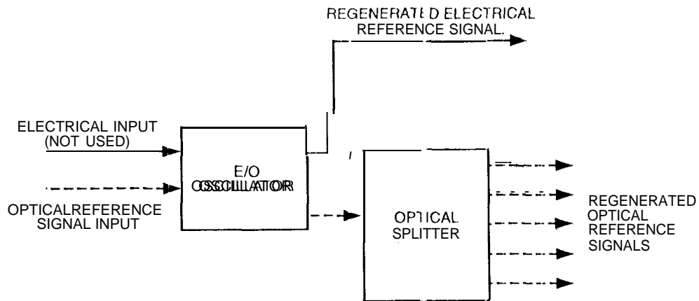
Fig. 13. Optical frequency reference regeneration and distribution.
