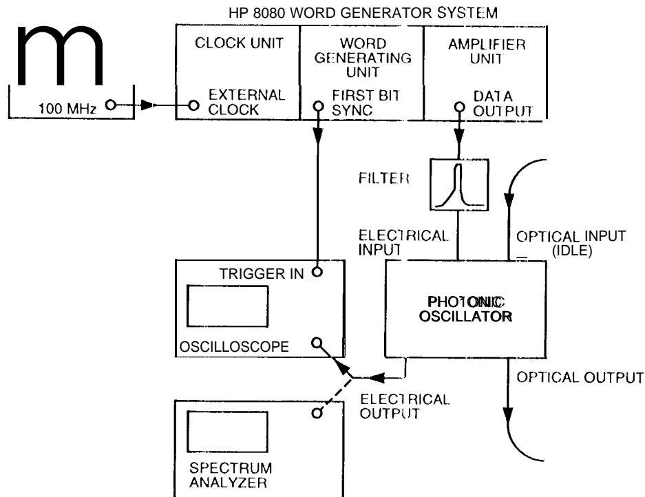
Fig. 2. Clock recovery experiment setup.
