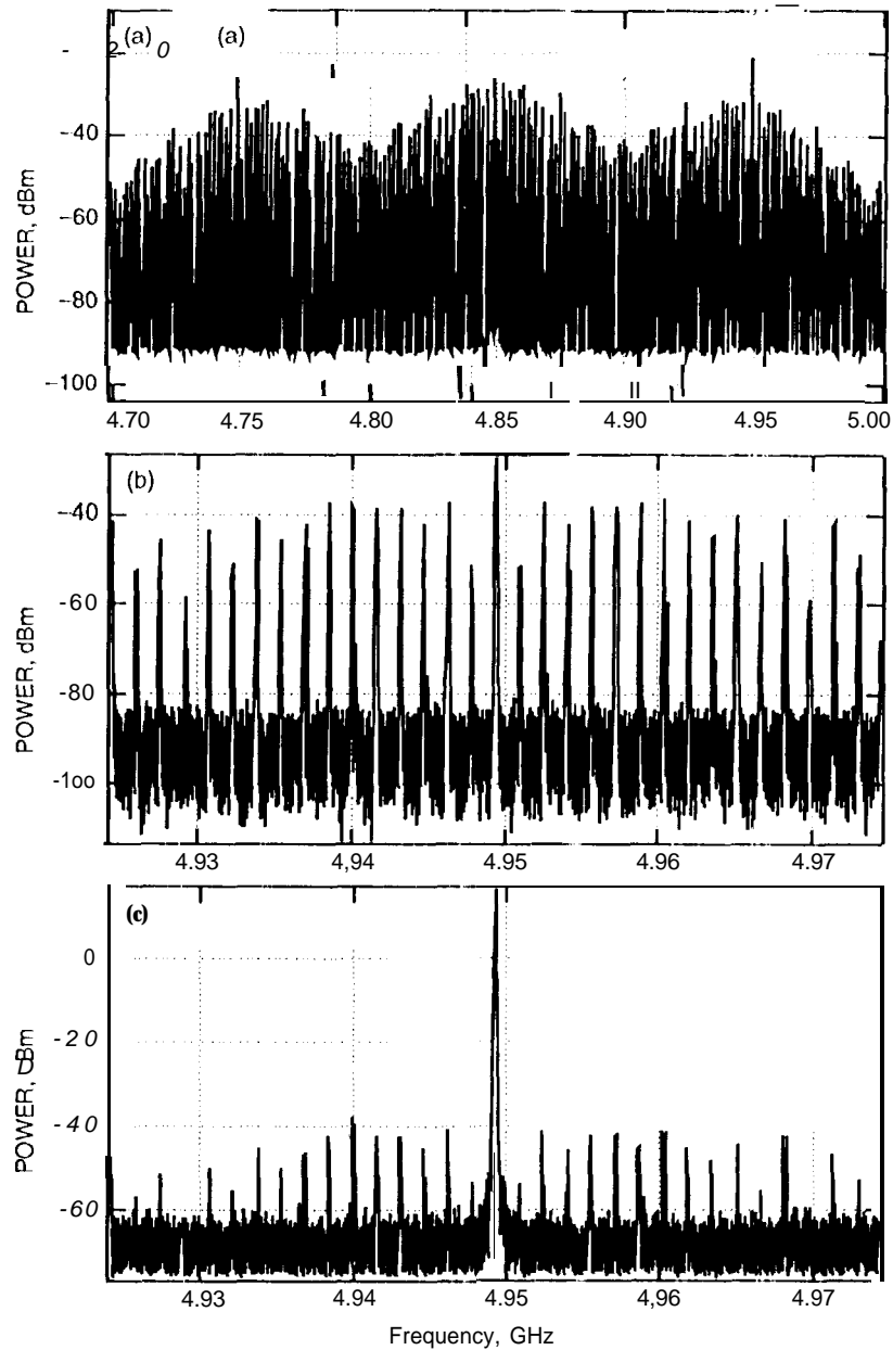
Fig. 8. The 4.95-GHz clock recovery from an RZ data stream measured in frequency domain: (a) up-converted data, (b) data input to the photonic oscillator, and (c) recovered clock.
