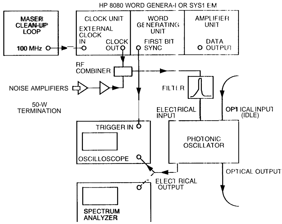
Fig. 9. Experiment setup for demonstrating photonic carrier recovery.
