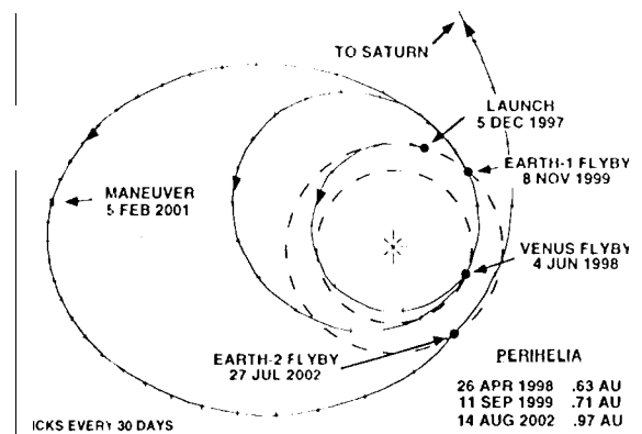
Fig. 5. VEEGA97 - Inner Solar System Trajectory.
