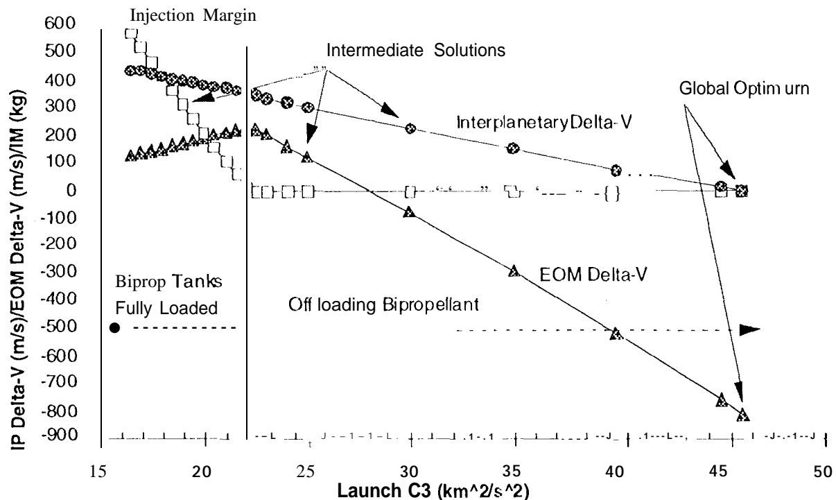
Fig. 2. Injection Margin, Interplanetary Delta-V, and Delta-V at End of Mission versus C_3 for Launch on 01/19/97, Arrival on 07/1/04.
