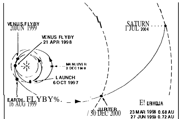
Fig. 1. Cassini-VVEJGA October 1997, Interplanetary Trajectory.
