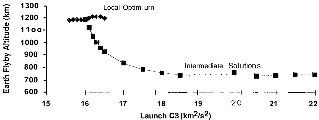
Fig. 4. Venus 1, Venus 2, and Earth Flyby Altitudes versus C_3 for Launch on 10/19/97, Saturn Arrival on 7/1/04.
