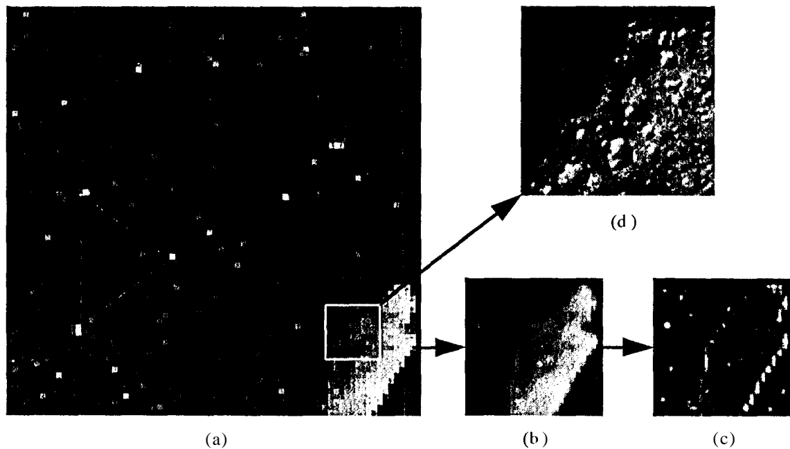
Figure 5. Combining a WFOV tracker with a NFOV science camera produces a powerful star and feature tracking system. (a) The WFOV system uses regional shuttering to track background stars and image extended objects. The extended object sub-image is processed (b) to allow feature tracking (c) used to point the NFOV science camera. The NFOV science camera (d) is free to collect data without the overhead of tracking responsibilities.
