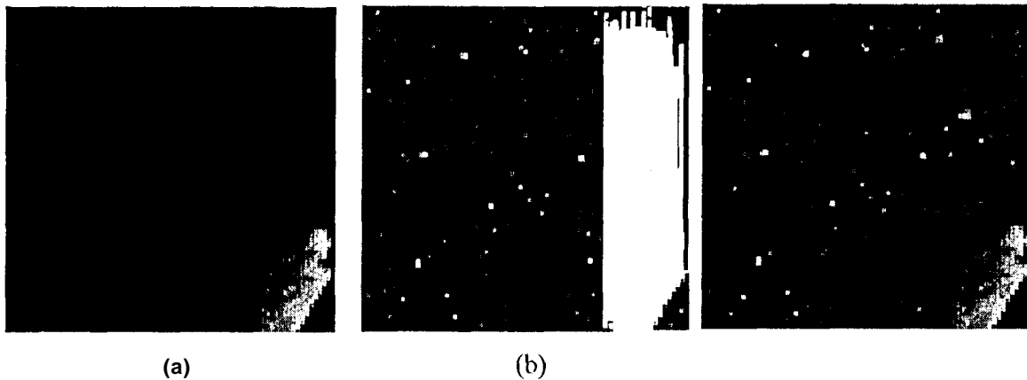
Figure 3. Application of a regional shutter concept to a simulated WFOV image containing both faint stars and a bright extended object. (a) Using a CCD, a short integration is required to properly record the extended object (bottom right) sacrificing background stars. (b) A sufficiently long integration brings out background stars but causes blooming across the image. (c) The APS regional shutter allows short integration times around the extended object and long integration for the stars.
