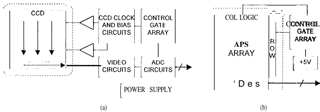
Figure 2. CCD array control (a) requires a sizable collection of analog and digital support circuits. In comparison, APS arrays can be controlled with a minimum set of components (b) due to their extensive on-focal plane electronics. Reducing total camera electronics component count shrinks circuit board size, reduces failure risks, and decreases overall power consumption.
