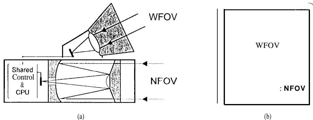
Figure 1. A compact and powerful star and feature tracking system is created by combining a narrow field of view (NFOV) science camera and a wide field of view (WFOV) star tracker. Both instruments use APS imaging arrays, share common electronics (a), and are optically co-aligned to observe a common region in the pointing direction (b).
