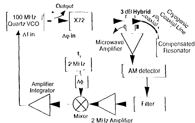
Figure 2. Pound (frequency lock) circuit with 2 MHz modulation frequency. Not shown is frequency offset circuitry associated with the x72 multiplier which derives the exact resonator frequency of 7.226 GHz.
