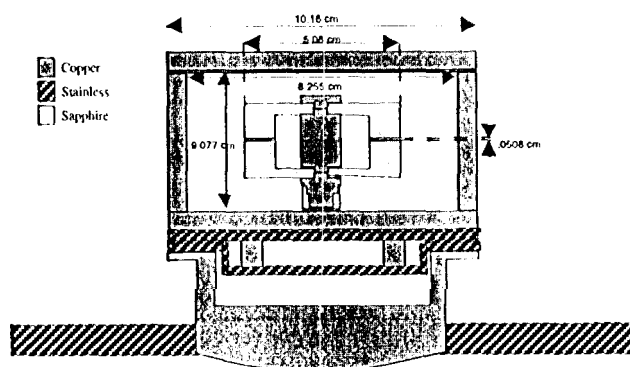
Figure 1. Compensated sapphire resonator with frequency turn-over temperature of \sim 87 K. Expansion of the copper center post with increasing temperature increases the gap spacing between the sapphire elements, counteracting an increase in dielectric constant in the sapphire. Stainless steel thermal isolation assembly reduces the effect of LN_2 temperature fluctuations.
