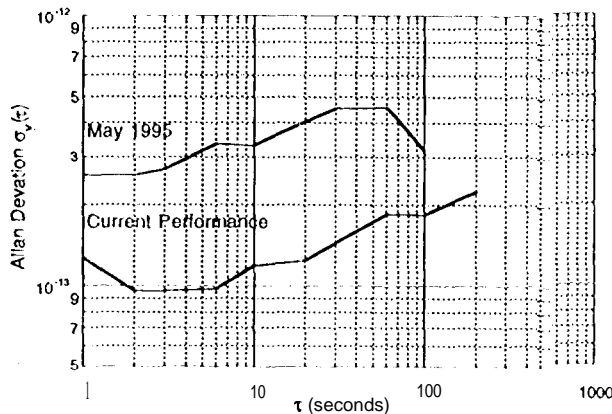
Figure 3. Allan Deviation of CSO frequency stability
