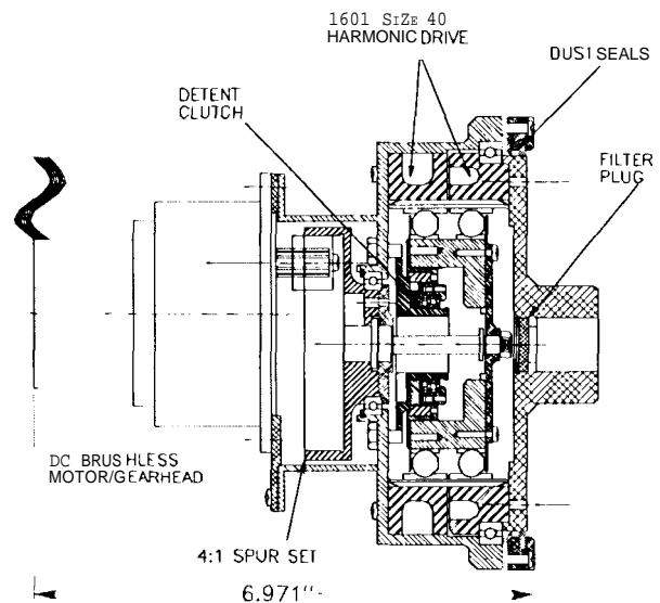
Figure 4: Lander Petal Actuator cross-section
