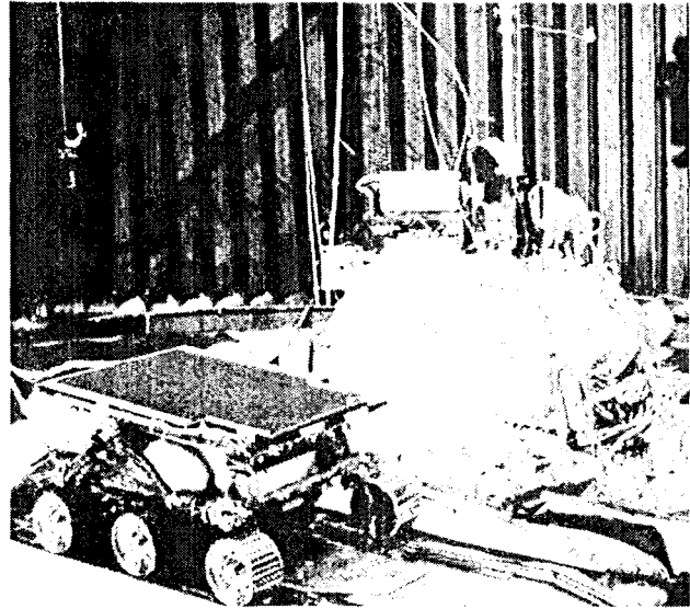
Figure 1: Mars Pathfinder Thermal test: IMP stowed, lander Petals, IMP and Ramp deployed
