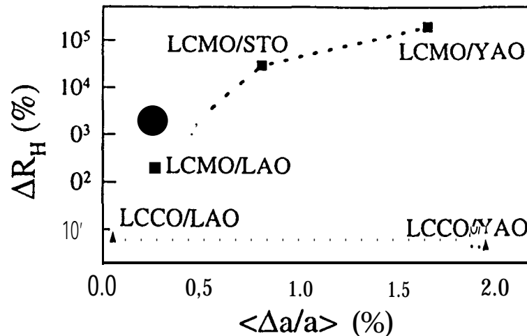
Fig. 1 Correlation of the magnetoresistance ( \Delta R_H ) and the substrate-induced lattice distortion in the manganites \text{La}_{0.7}\text{Ca}_{0.3}\text{MnO}_3 (LCMO). For comparison, the insignificant effect of lattice distortion on the magnetoresistance of the cobaltites \text{La}_{0.5}\text{Ca}_{0.5}\text{CoO}_3 (LCCO) is also illustrated.
