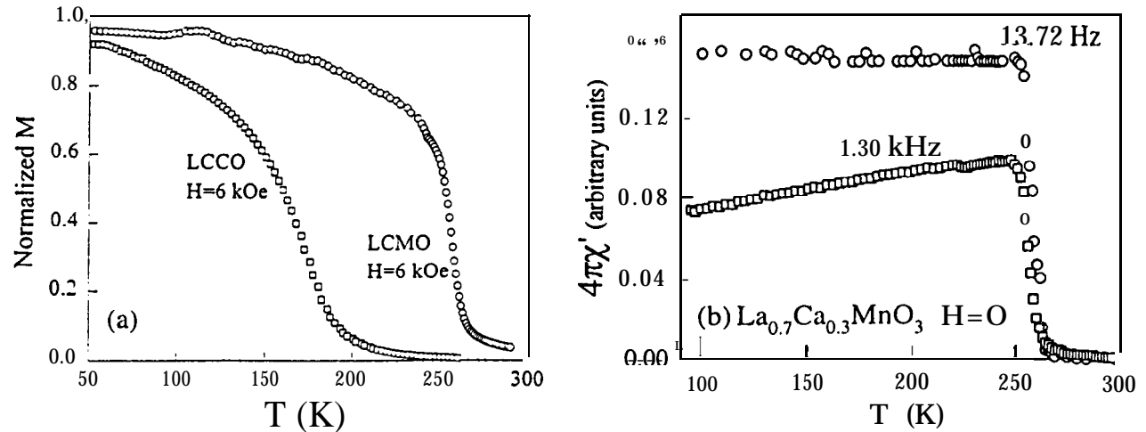
Fig.5 (a) The magnetization ( M ) vs. temperature ( T ) data for bulk LCMO and LCCO samples. (b) The real part of the ac magnetic susceptibility ( 4\pi\chi' ) vs. temperature ( T ) data taken at frequencies f = 13.72 Hz and f = 1.30 kHz and for H = 0 .
