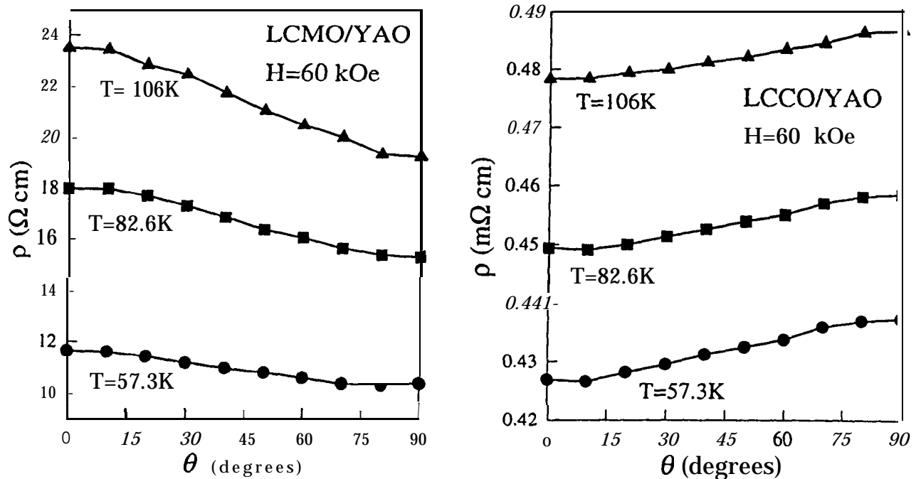
Fig.4 The anisotropic resistivity of LCMO/YAO and LCCO/YAO films at various temperatures below T_C and for H = 6 Tesla.
