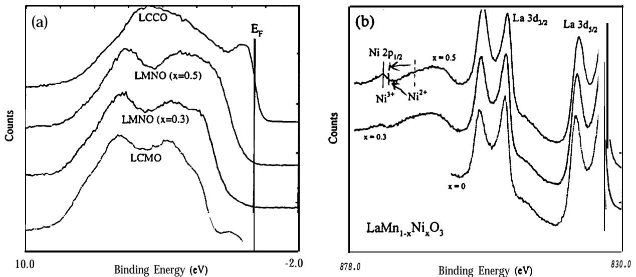
Fig.2 (a) The room-temperature valence band spectra of the LCMO, LCCO and LMNO films on LAO substrates. We note the absence of any density of states at the Fermi level for the LCMO and LMNO, and a high density of states at the Fermi level for the LCCO. (b) The La 3d and Ni 2p signals of the \text{LaMn}_{1-x}\text{Ni}_x\text{O}_3 ( x = 0, 0.3, 0.5 ) films. We note that the La 3d signal reflects strong mixing of final states with \underline{3d^9 4f^0 L} and \underline{3d^9 4f^1 L} character, and that the Ni 2p_{1/2} signal occurs at a binding energy of 872.2 eV, consistent with \text{Ni}^{3+} as measured in \text{LaNiO}_3 [19].
