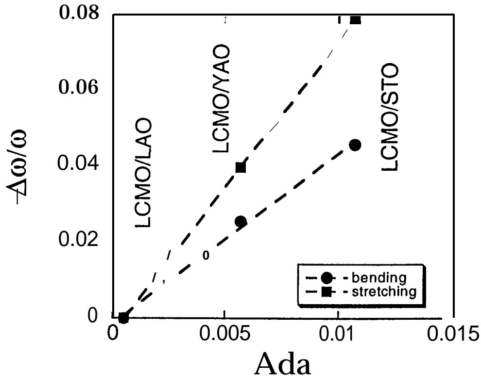
Fig.6 Correlation of the ratio of the phonon frequency shift ( -\Delta\omega/\omega ) and the substrate-induced lattice strain ( \Delta s/a ) for the Mn-O stretching and Mn-O-Mn bending modes in LCMO epitaxial films[17].
