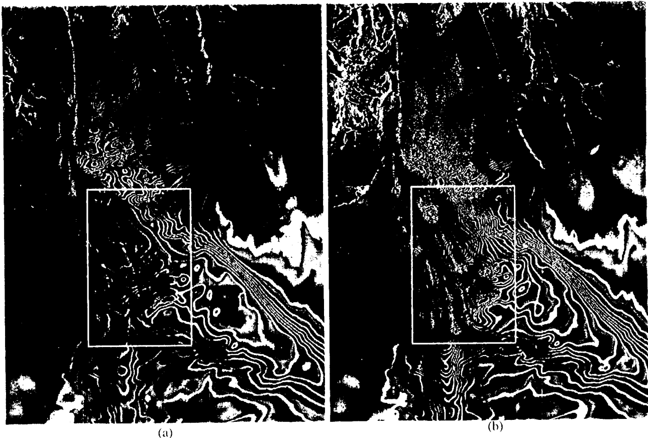
Figure 3. Interferograms from the fast moving area of the Ryder Glacier (a) before (21-22 September 1995) and (b) during (26-27 October 1995) a mini surge. Each fringe is equivalent to 7.2 cm of horizontal displacement in the across track direction or 3.0 cm of vertical displacement. Both interferograms were acquired from data collected along the same descending track.
