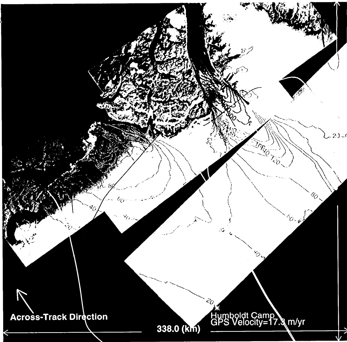
Figure 1. Contour map of the across-track component of velocity for the Petermann and Humboldt Glaciers for the area indicated by a white rectangle in Figure 1. The across track direction is slightly different for each swath. The approximate across track direction is indicated by an arrow in the lower left corner. Contour interval is 20 m/yr for velocity less than 200 m/yr and is 100 m/yr for values greater than 200 m/yr. Red lines indicate locations of CoRDS profiles.
