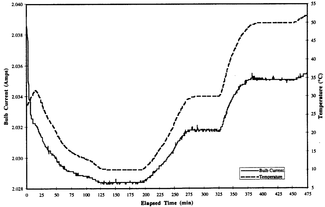
Figure 6. Bulb Current and Temperature vs. Elapsed Time
