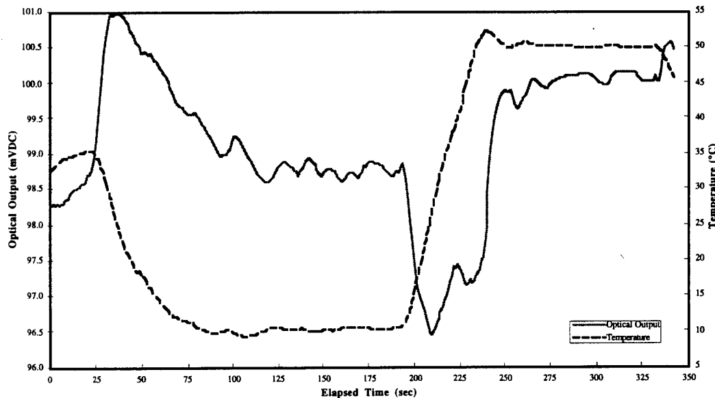
Figure 3. First Run: Optical Output and Temperature vs. Time for OBC without a shear plate
