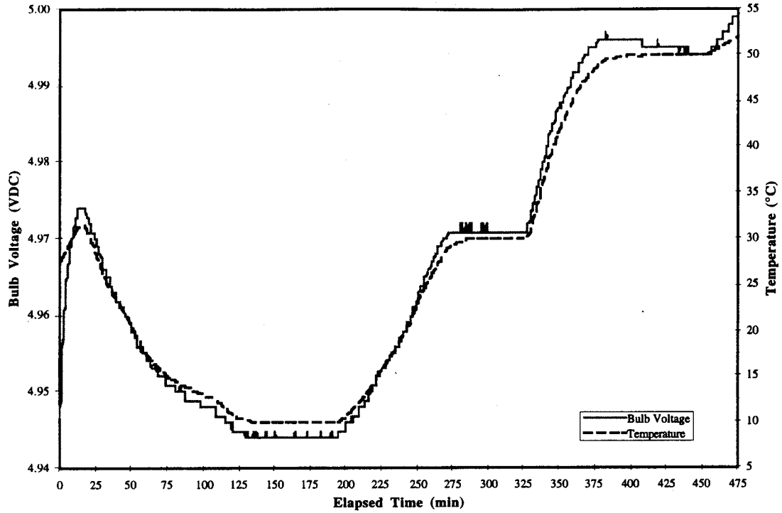
Figure 5. Bulb Voltage and Temperature vs. Elapsed Time
