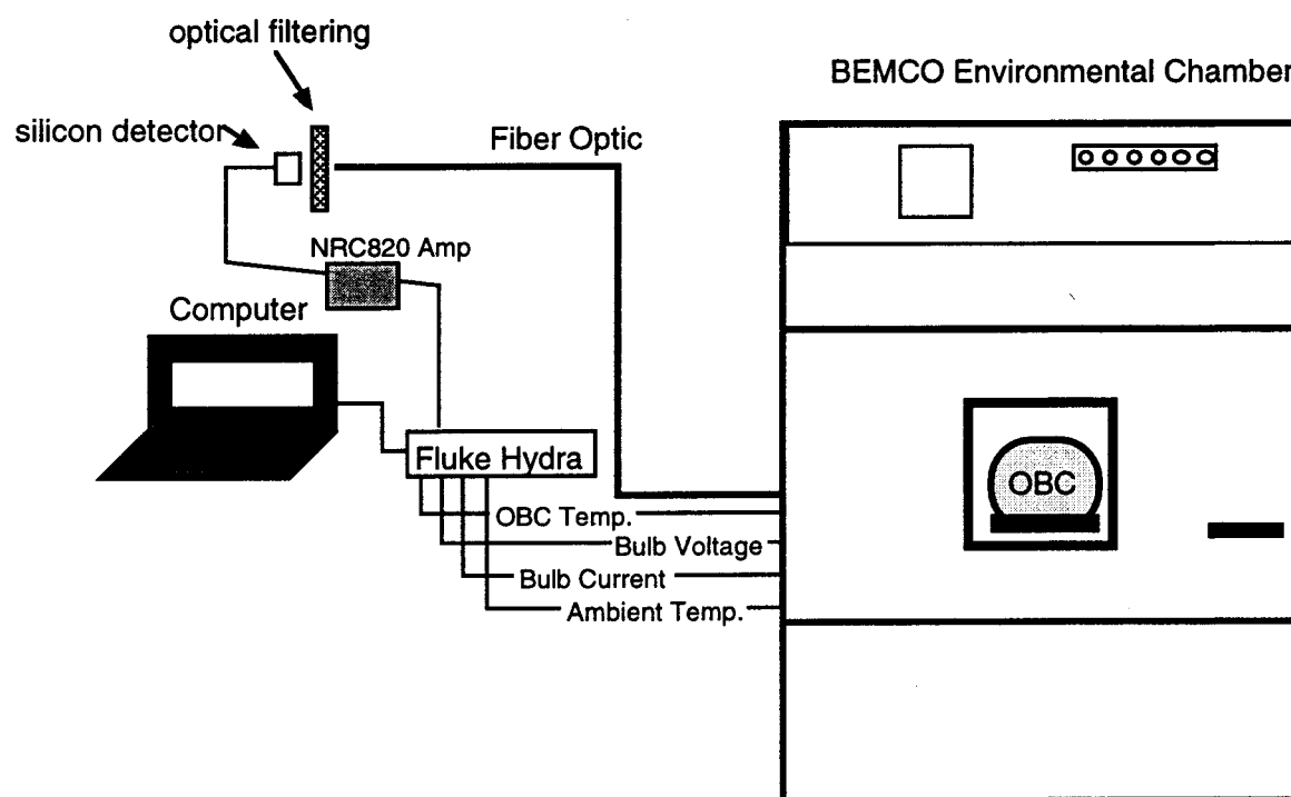
Figure 2. Experimental Set-Up
