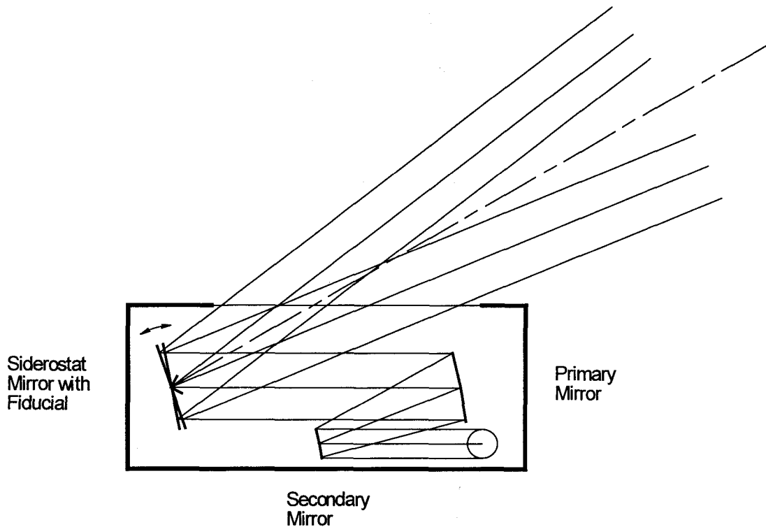
Figure 4 SIM Classic Siderostat Bay
