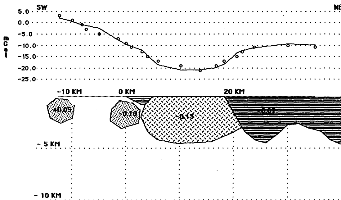
FIGURE 2. Two and half dimensional gravity model of the Teague Ring structure. Profile is oriented in a northeast-southwest direction. Small circles indicate measured gravity values; the line indicates the modeled gravity. Numbers denote the relative densities for the bodies in \text{g cm}^{-3} relative to the basement. Horizontally striped bodies are Earraheedy Group rocks; the stippled body represents the low-density core material; shaded bodies represent density anomalies within the crystalline crust. Vertical exaggeration is 2X.
