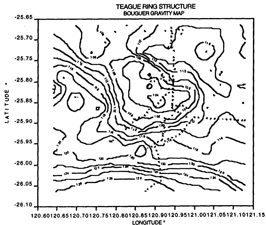
FIGURE 1. Simple Bouguer gravity map of the Teague Ring structure. Contour interval is 2 mGal. Crosses indicate station locations.
