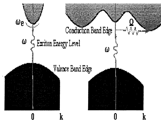
Figure 1. Band structure of semiconductor device materials including excitons.
