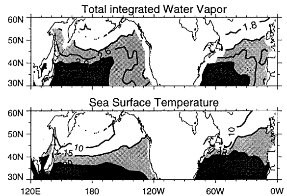
FIG. 3. The top panel is the total integrated water vapor from SSM/I measurements, contour level is 0.4 \text{ g/cm}^2 , values greater than 2.2 \text{ g/cm}^2 and 3.0 \text{ g/cm}^2 are denoted by light and dark shading, respectively. The bottom panel is the sea surface temperature from AVHRR, contour level is 5^\circ\text{C} , values greater than 15^\circ\text{C} and 20^\circ\text{C} are denoted by light and dark shading, respectively. Data are monthly average in July 1992.
