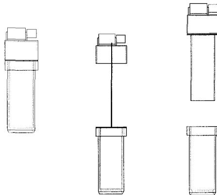
Figure 5: Penetrator Barrel, Firing and Retrieval System, displaying sampling sequence
