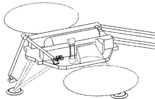
Figure 2: MSR Lander with RA and Scoop End Effector
