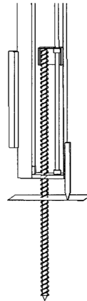
Figure 1: Deedri Drill Box System
